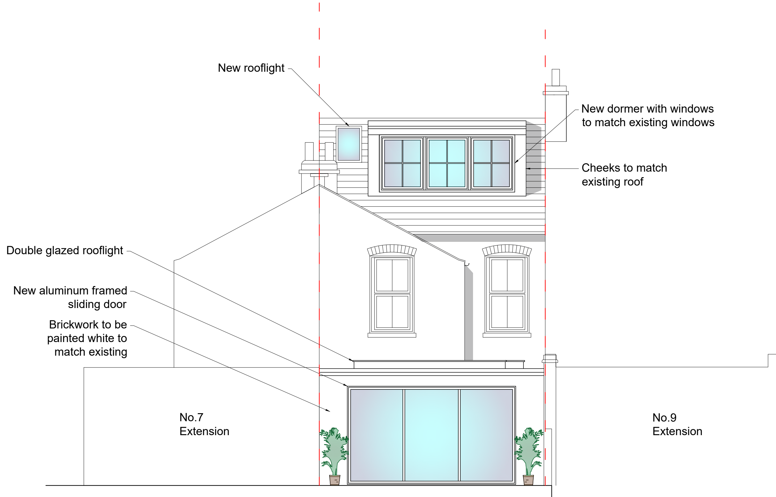
Rear Elevation
