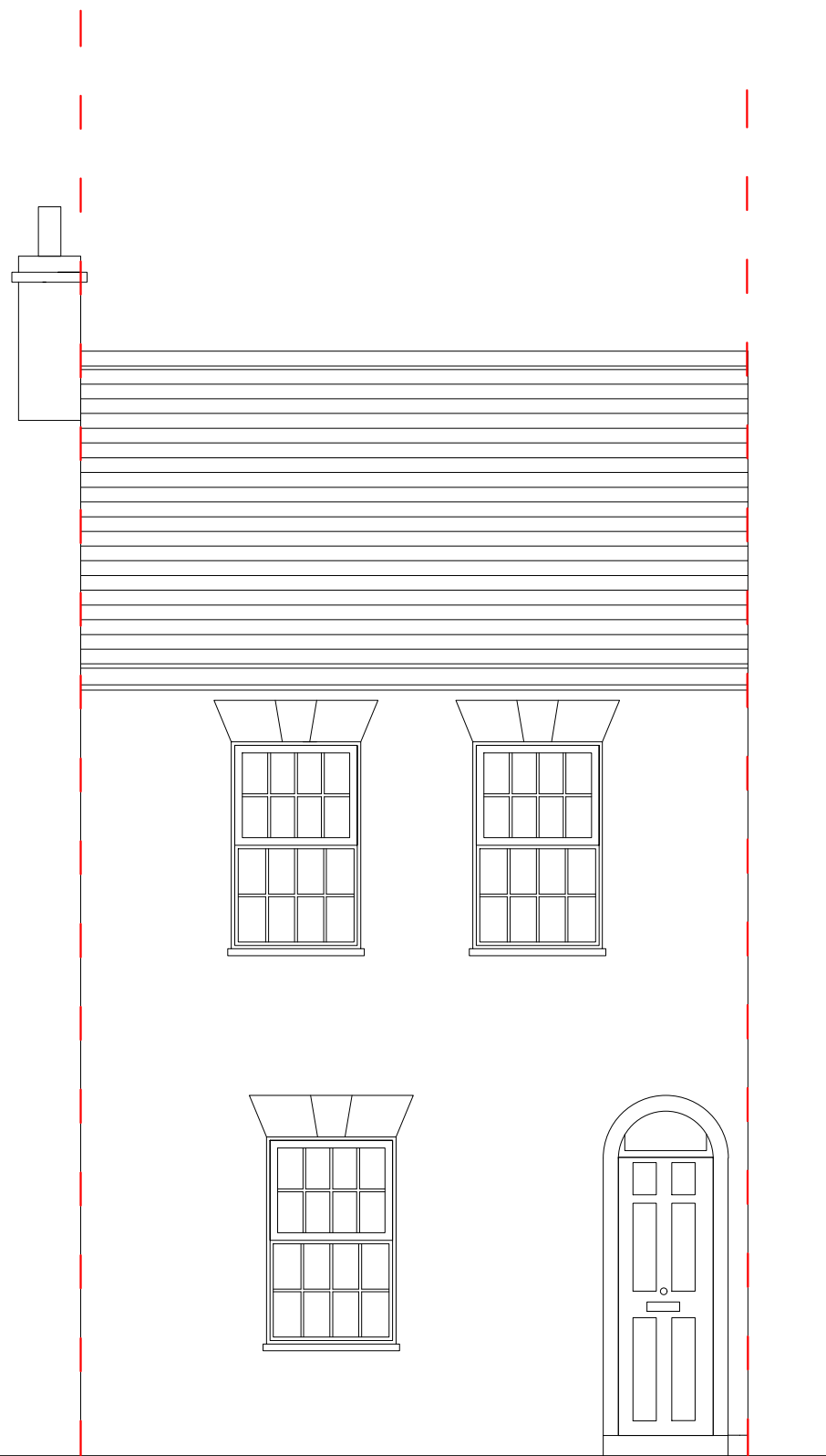
Front Elevation
