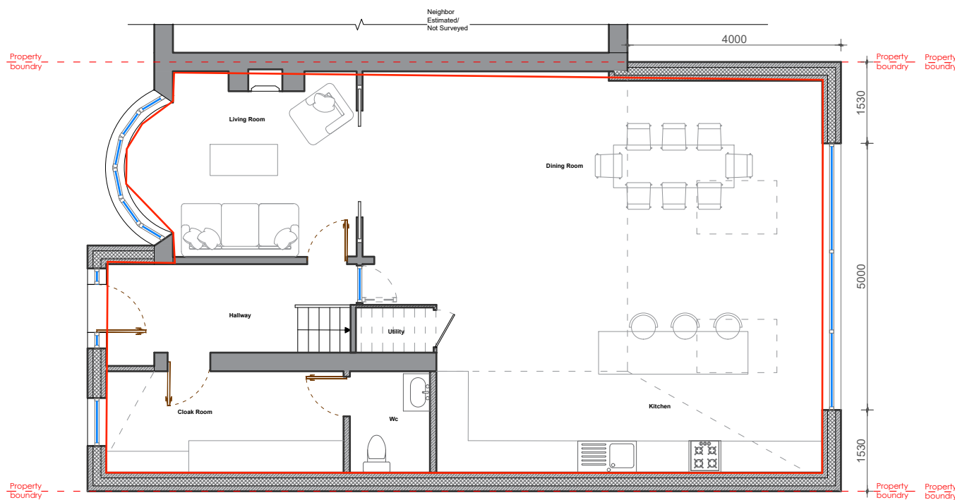
Proposed Ground 1:100
