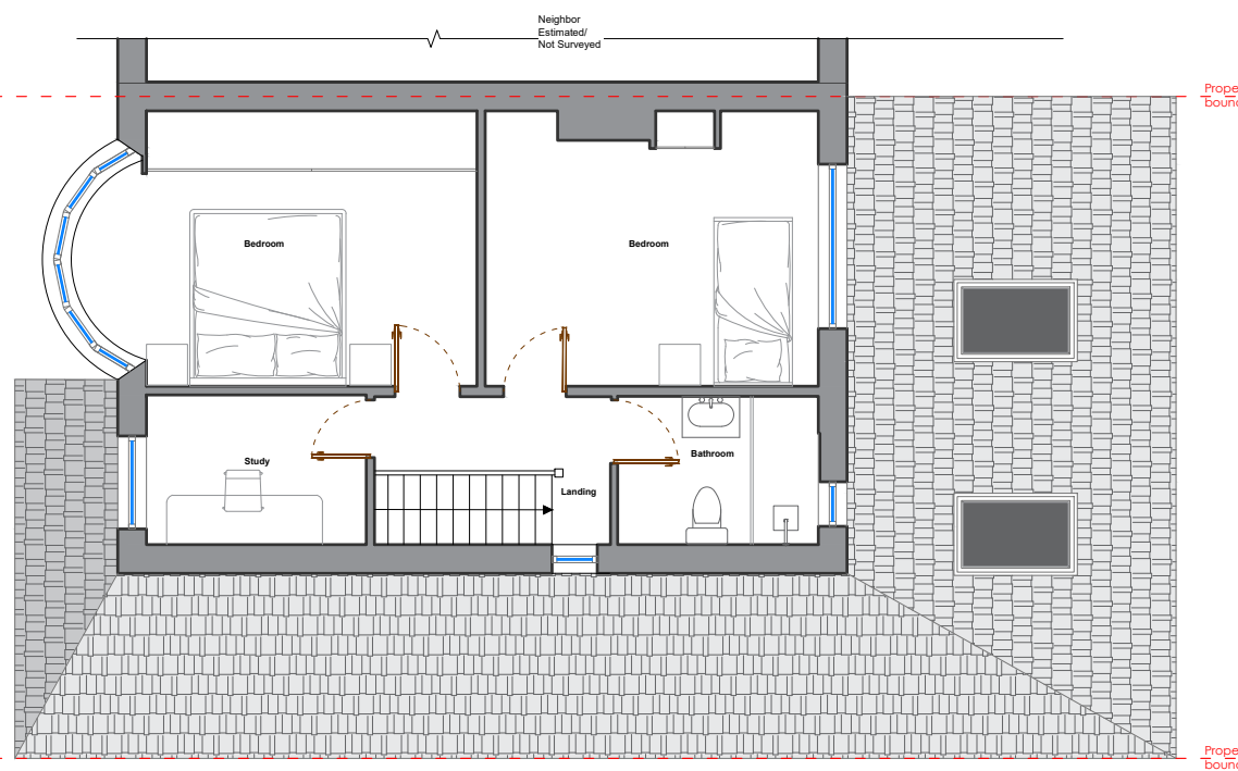
Proposed First 1:100
