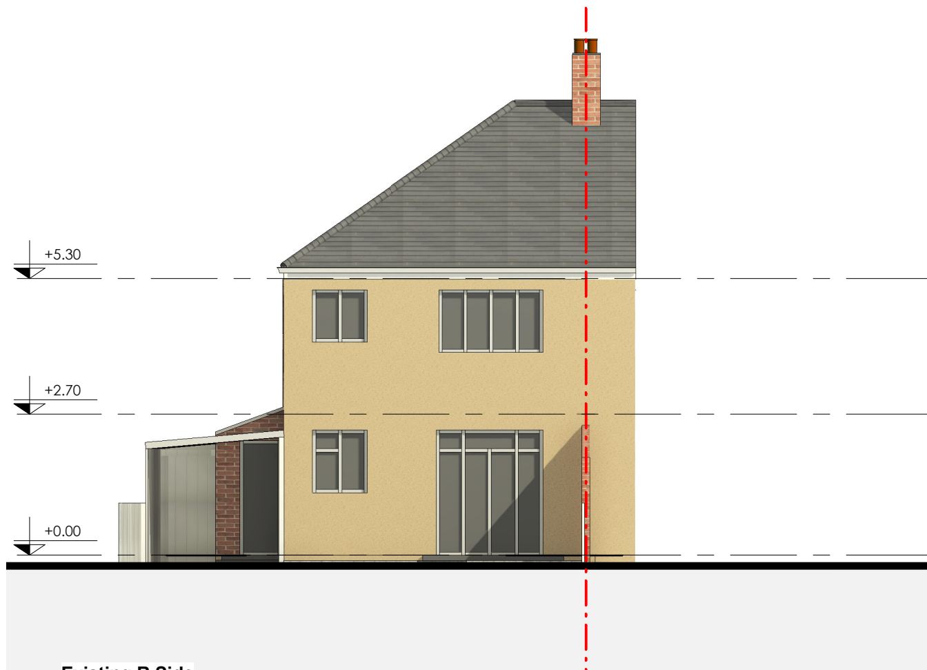
Existing R Side 1:100
