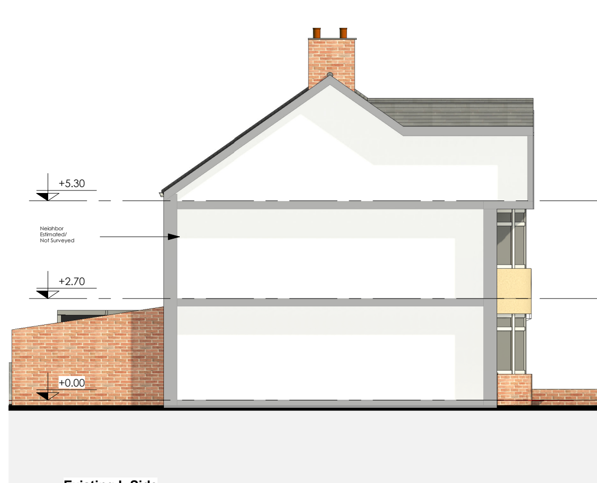
Existing L Side 1:100
