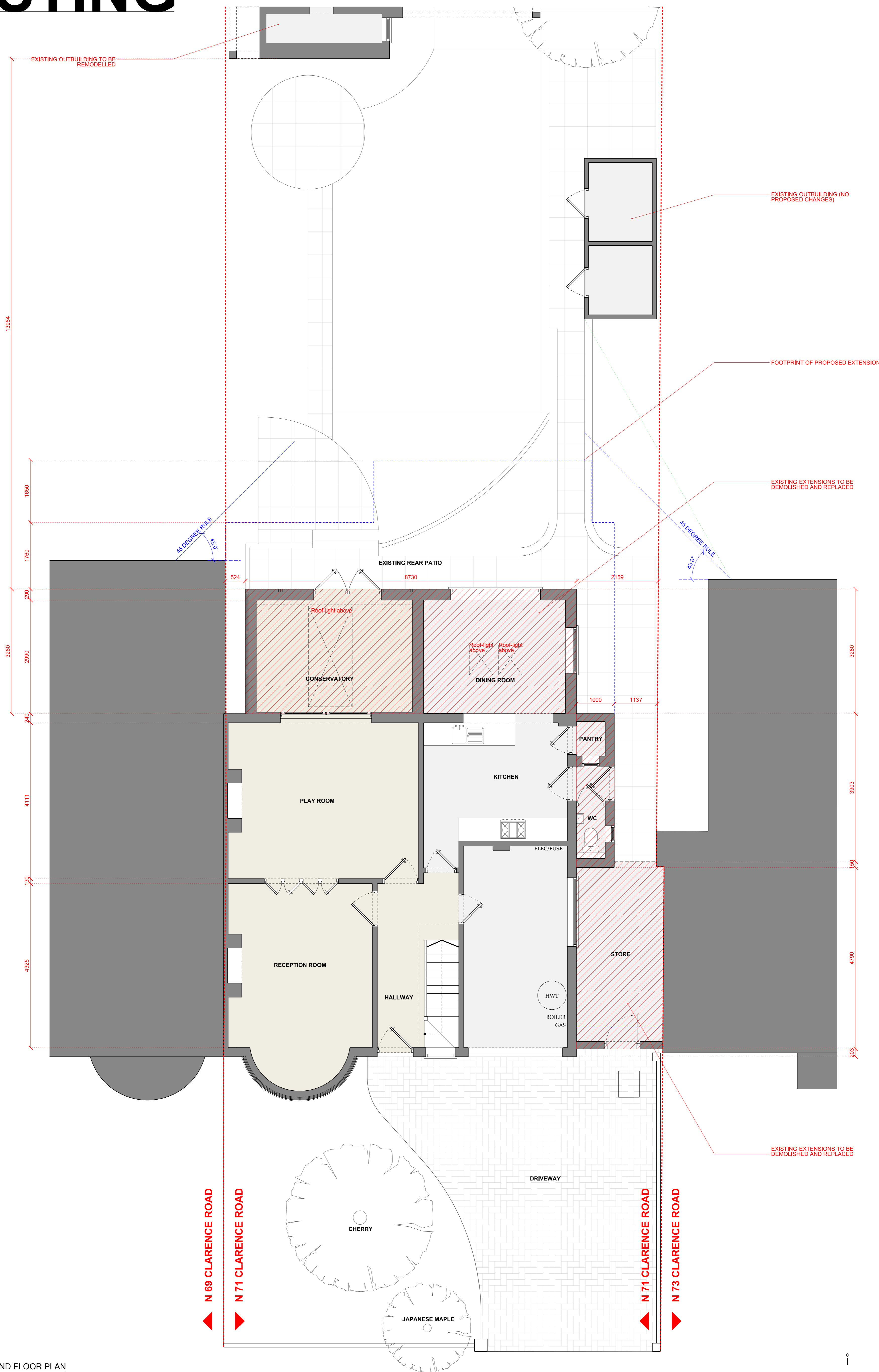
1 GROUND FLOOR PLAN 101 EXISTING 1:50
