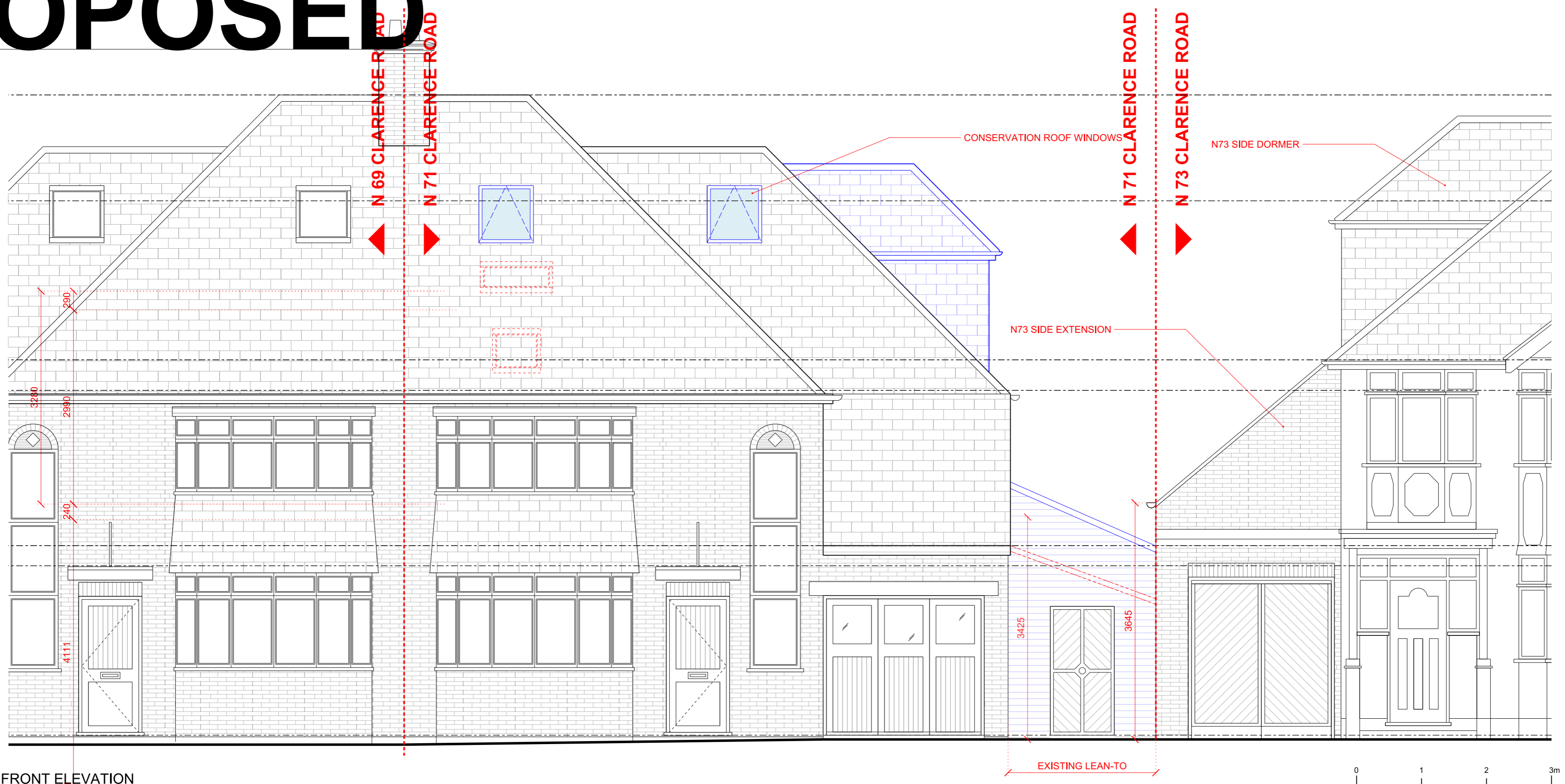
1 300 FRONT ELEVATION PROPOSED 1:50
