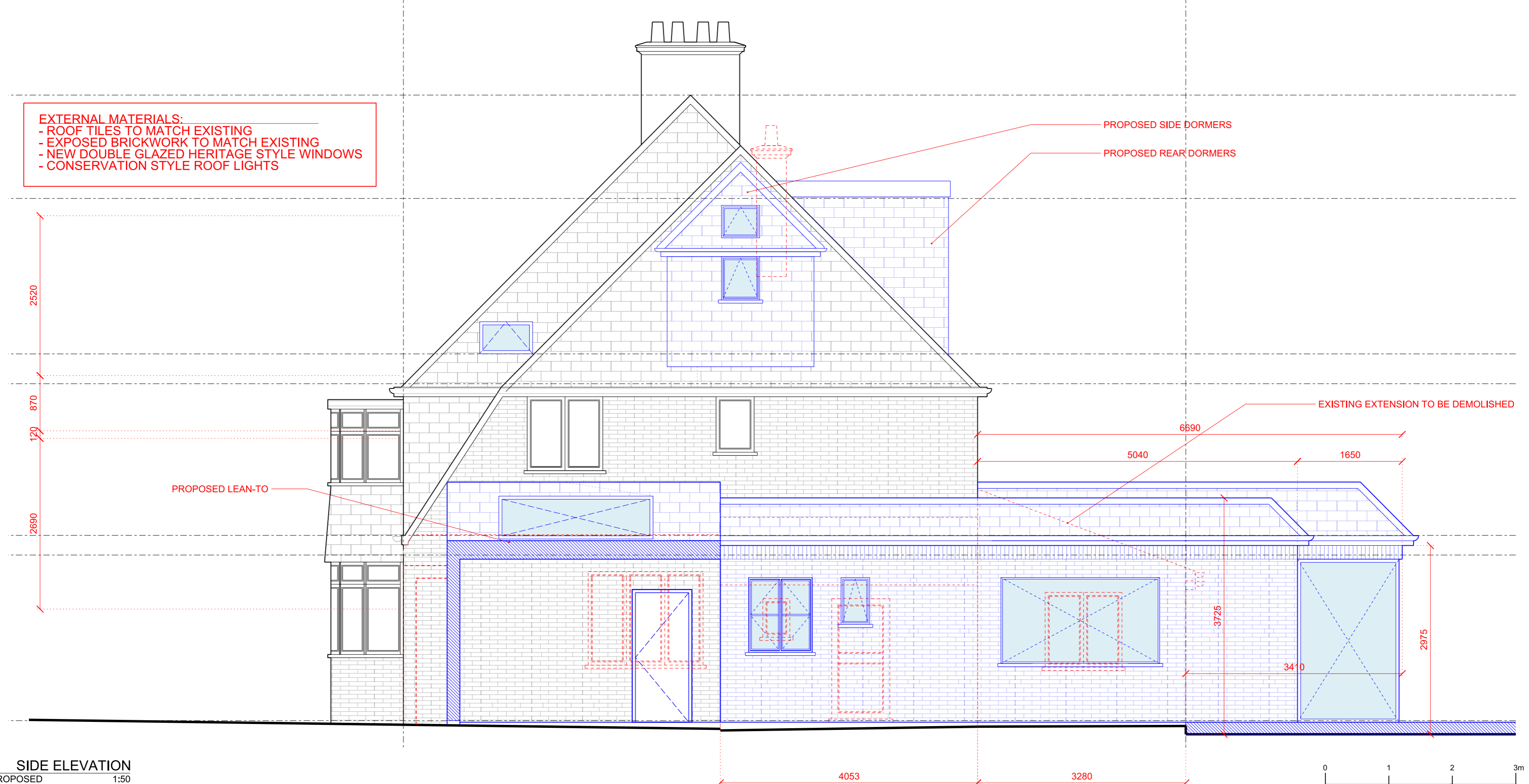
2 300 REAR ELEVATION PROPOSED 1:50
