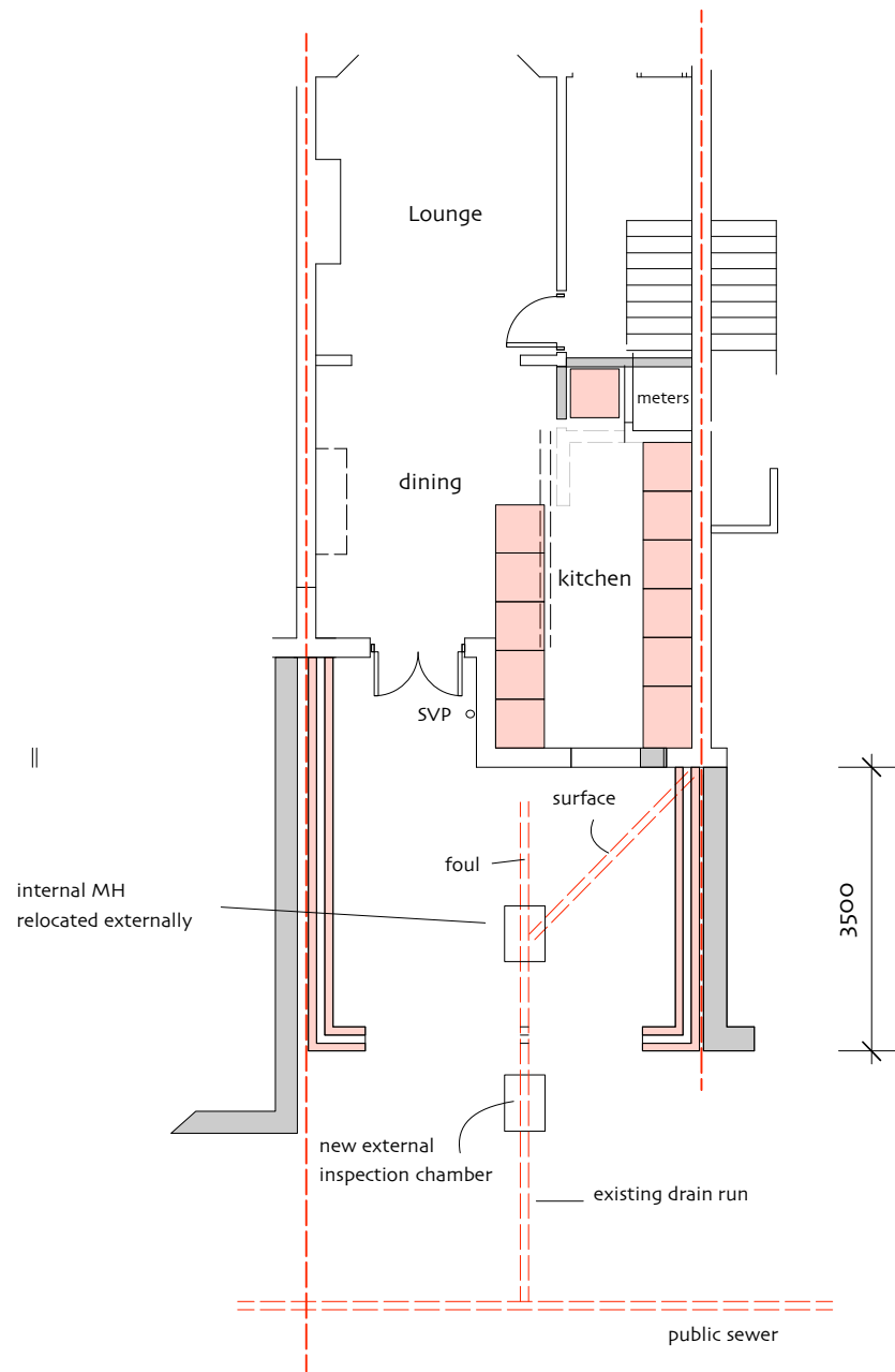
GROUND FLOOR
