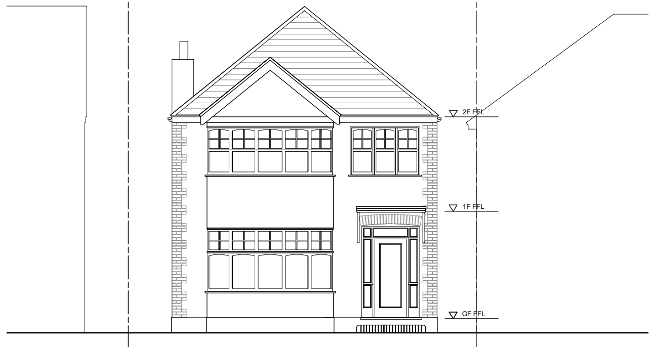
01 Existing Front Elevation 1:100 @ A3
