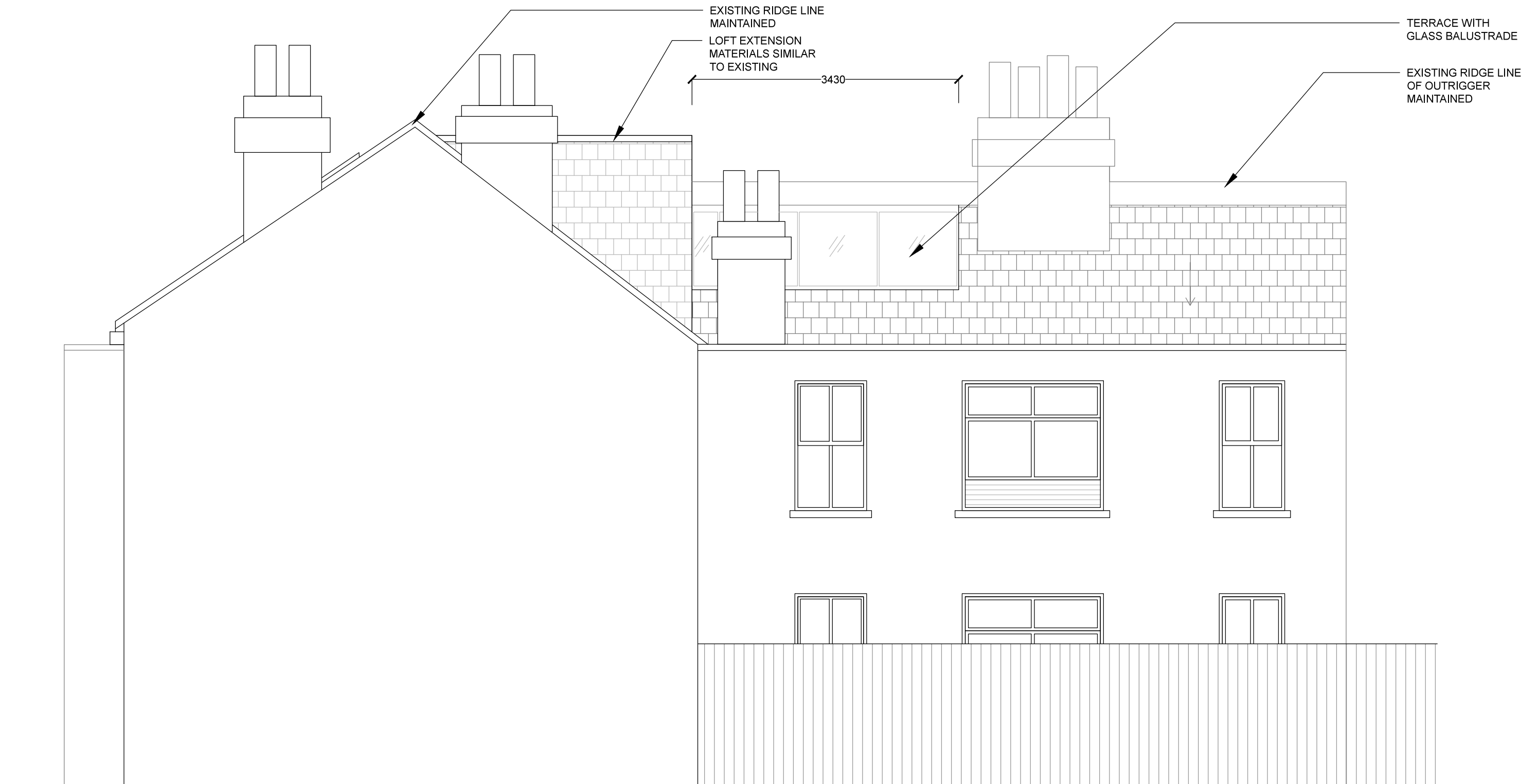
PROPOSED SECTION
