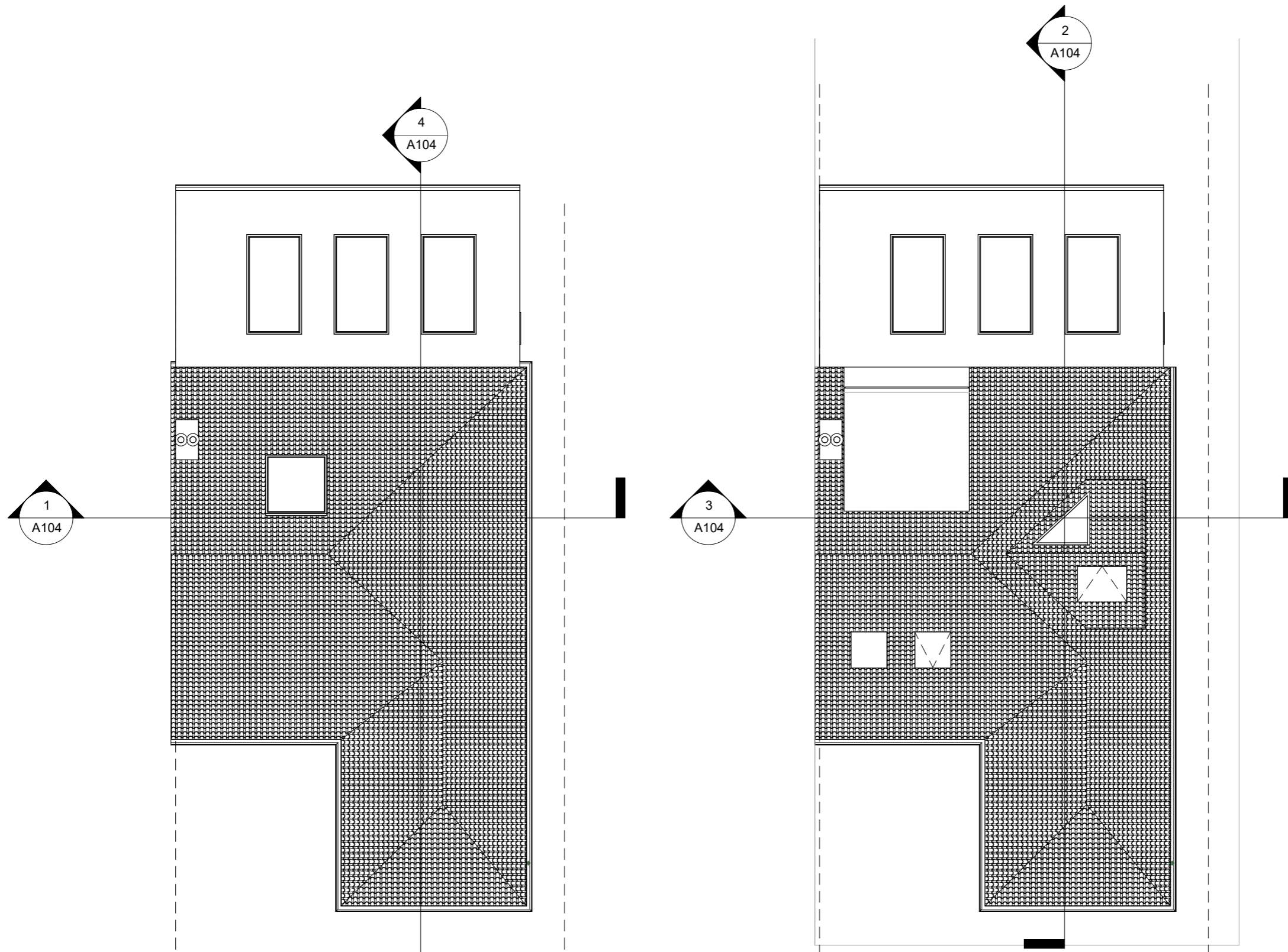
1 Roof - Existing 1 : 100
