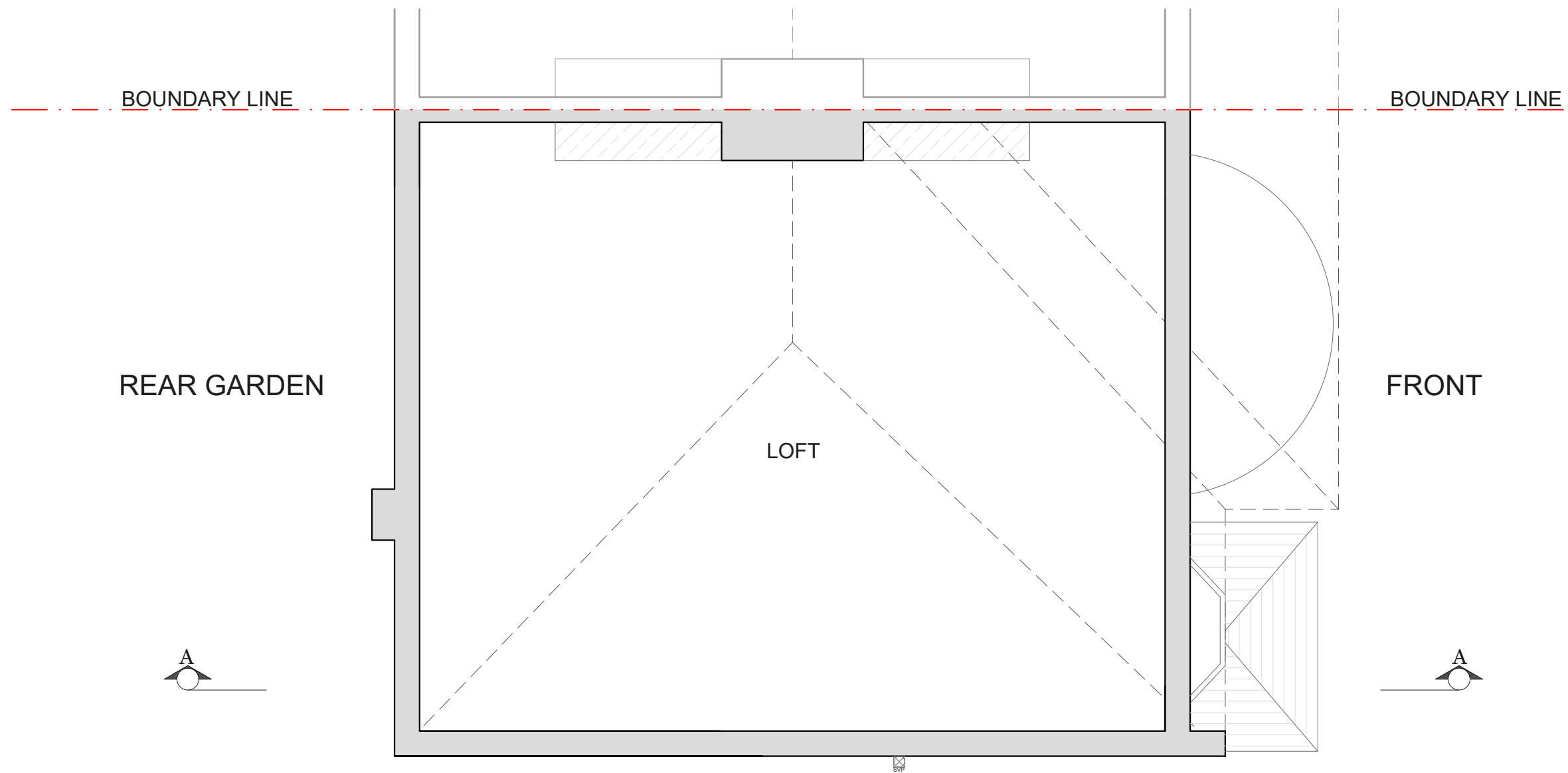
EXISTING LOFT FLOOR PLAN SCALE 1:50
