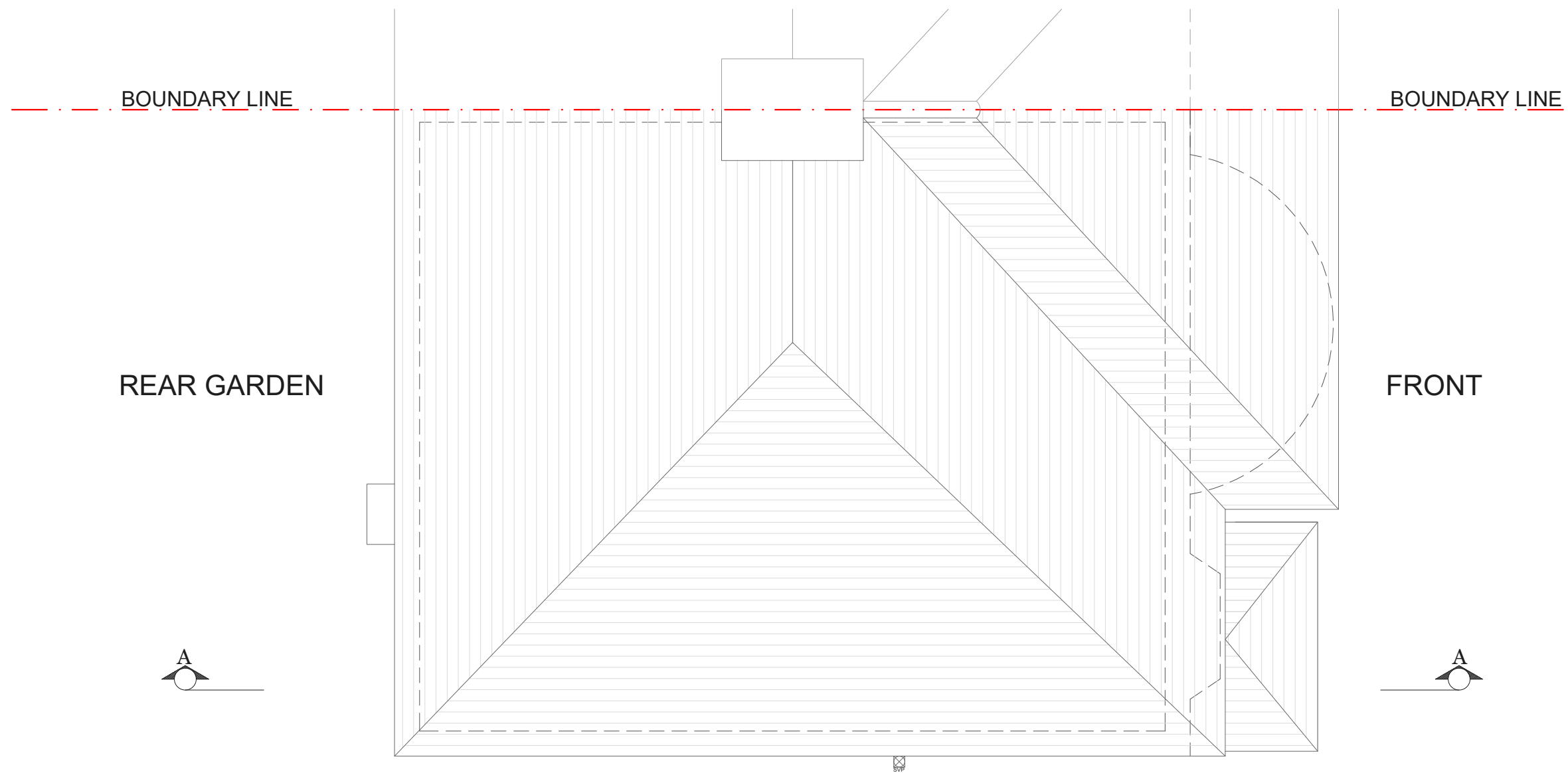
EXISTING ROOFTOP PLAN SCALE 1:50
