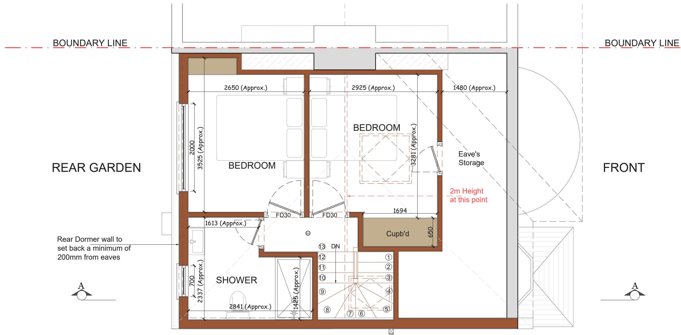
PROPOSED LOFT FLOOR PLAN SCALE 1:50
