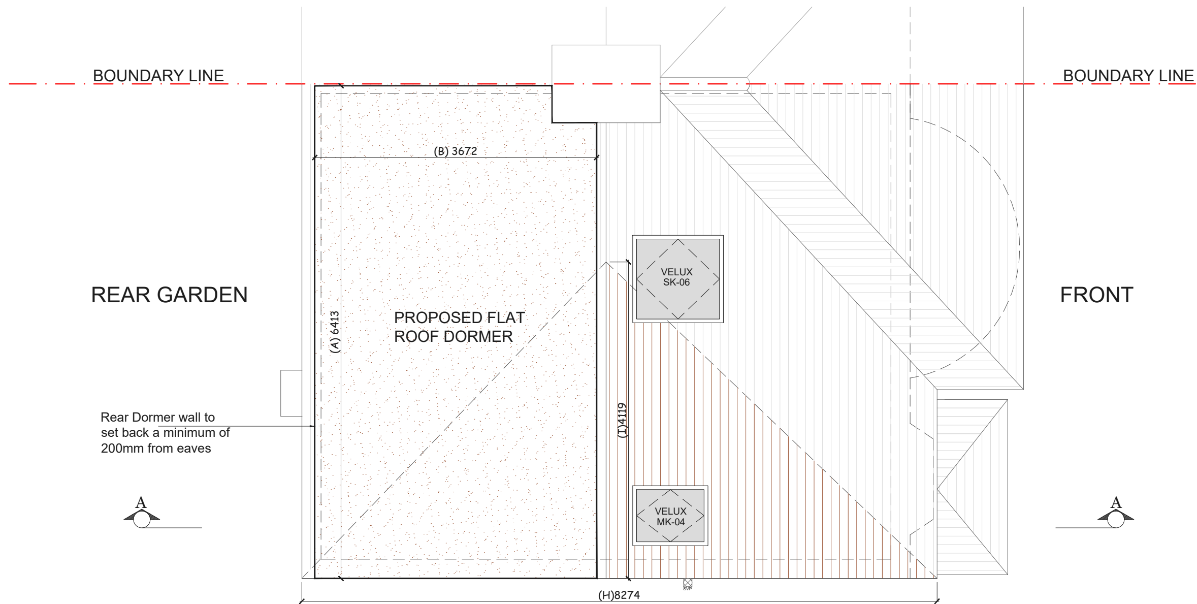
PROPOSED ROOFTOP PLAN SCALE 1:50
