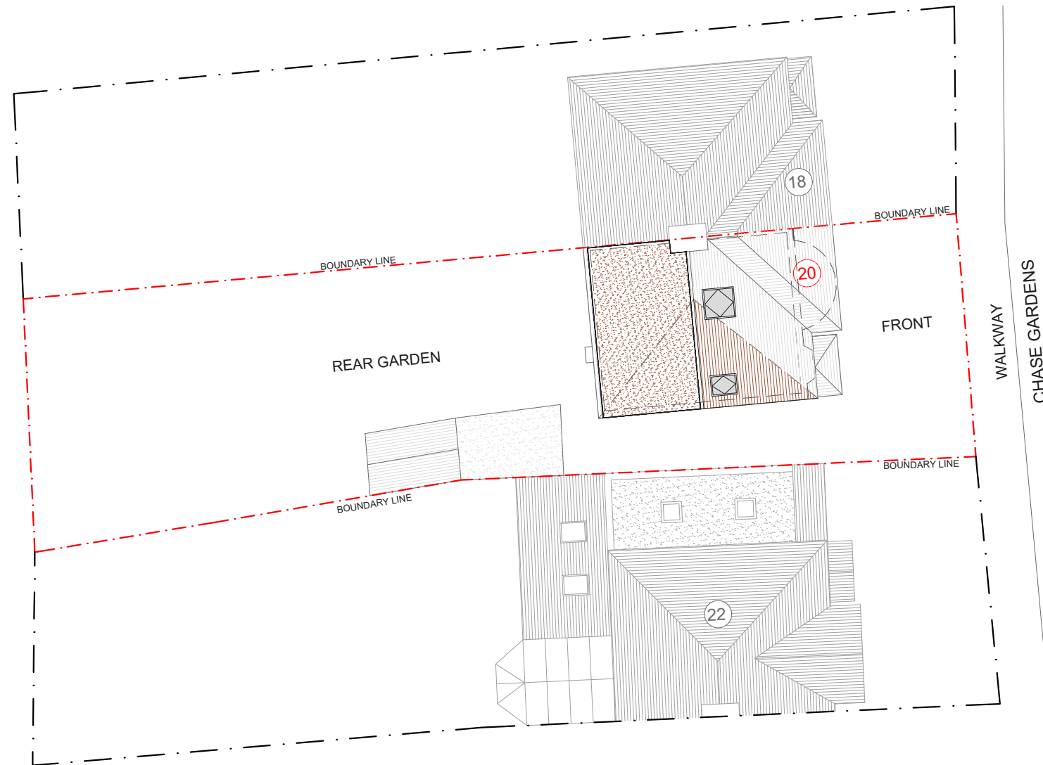
PROPOSED SITE / BLOCK PLAN SCALE 1:200
