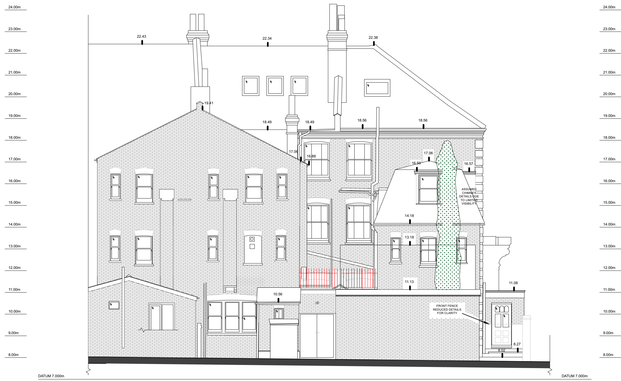
ELEVATION NO.2
