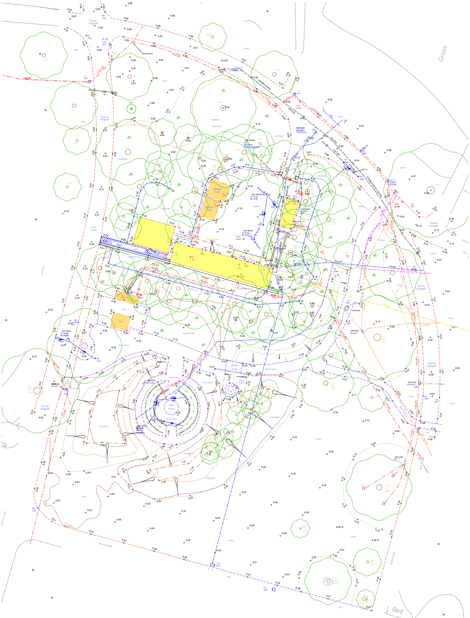
Existing Levels and Services Plan Drawing ref. RBG-24-007-001
