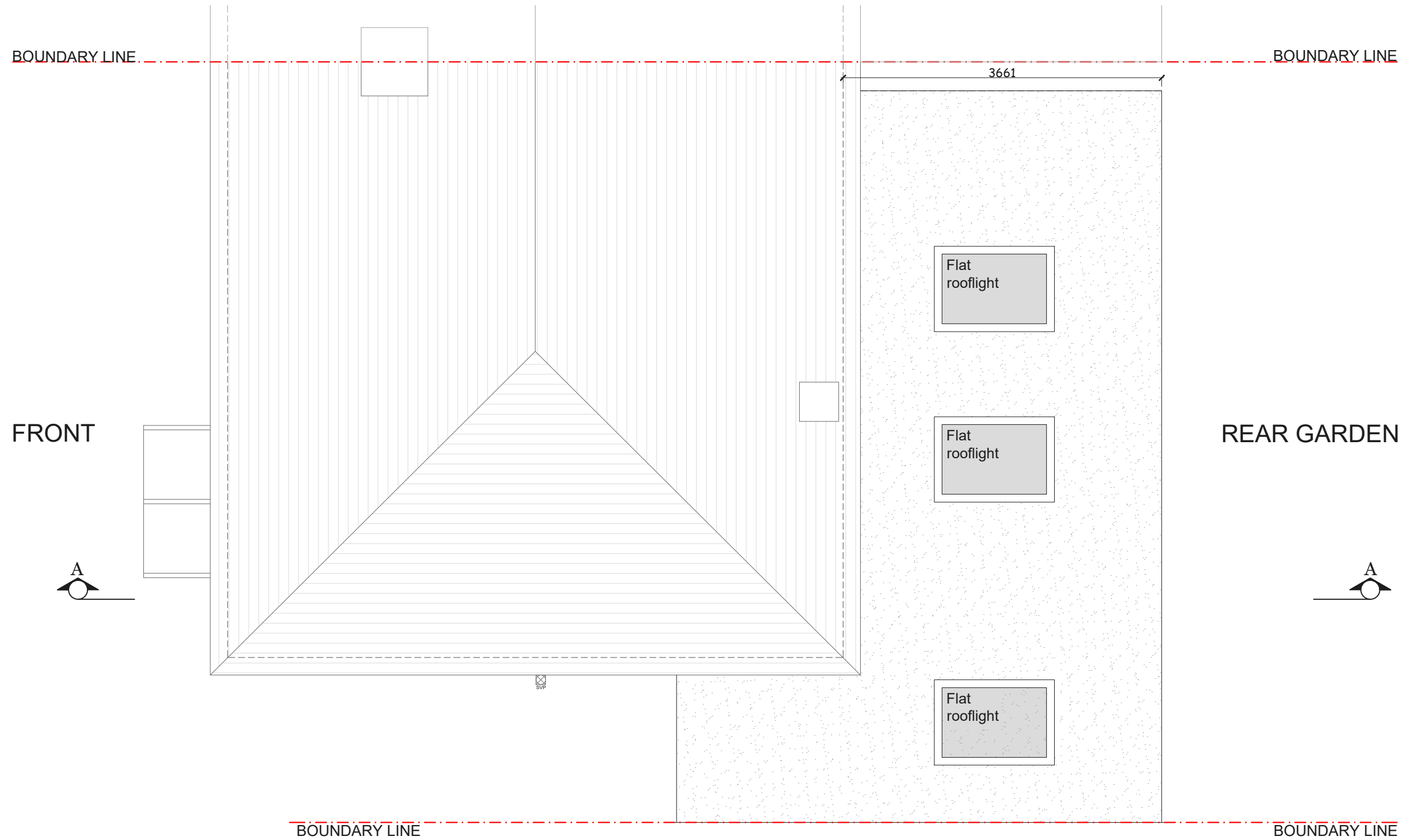
PROPOSED ROOFTOP PLAN SCALE 1:50
