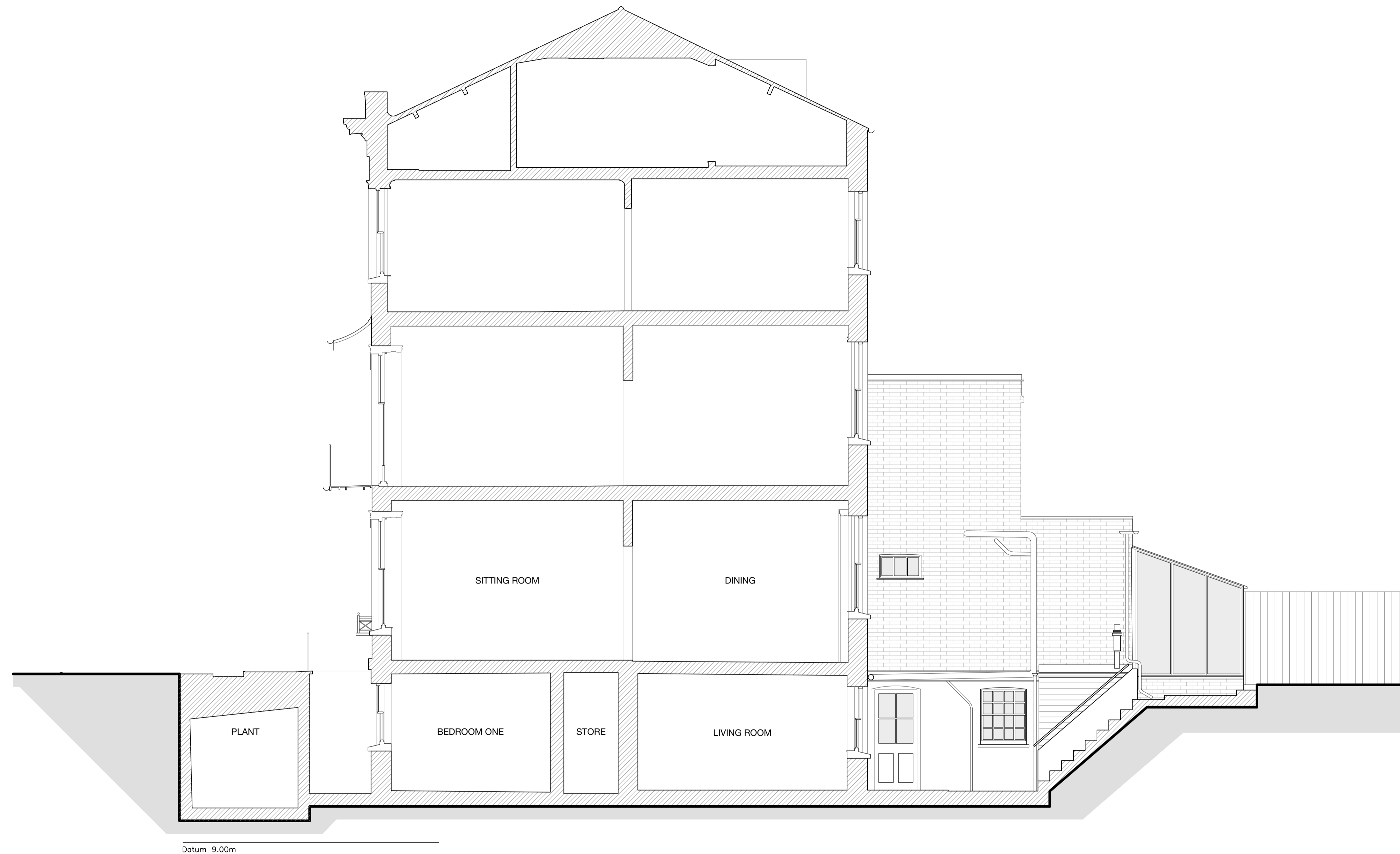
1 EXISTING SECTION A
