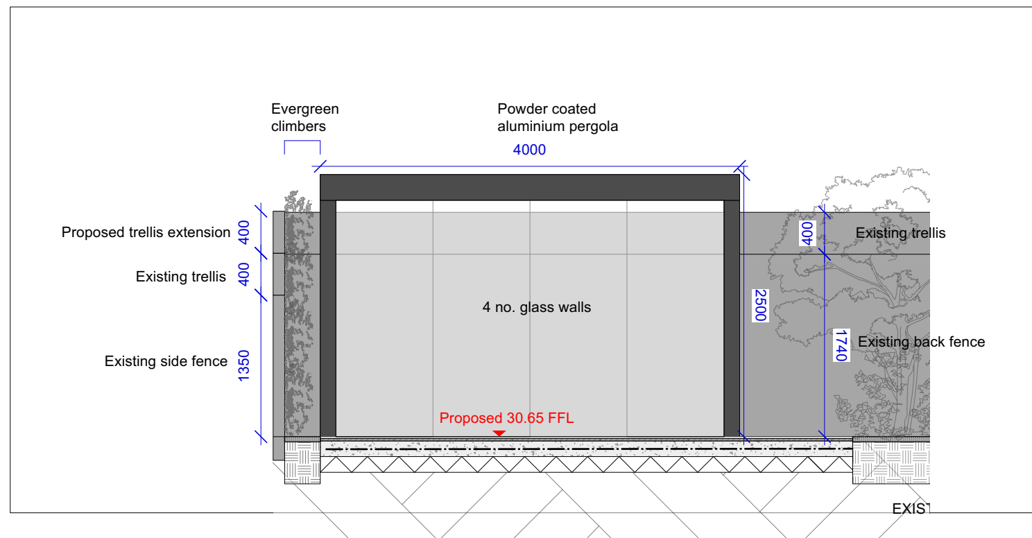
1 Proposed pergola elevation: view from house Scale: 1:50
