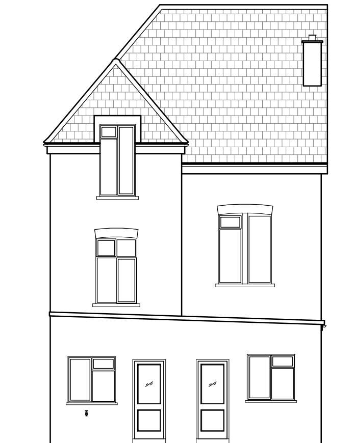
01 Existing Rear Elevation 1:100 @ A3
