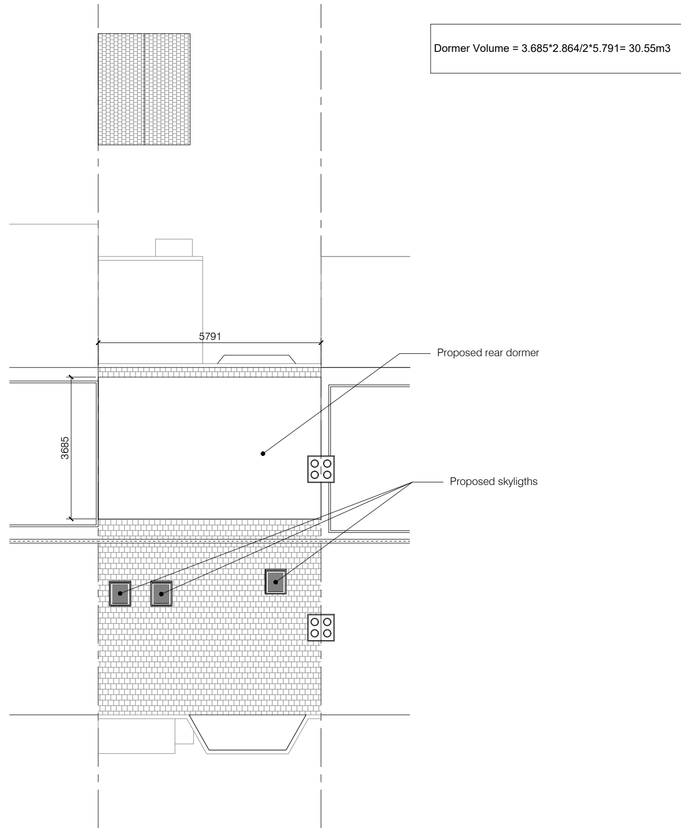
01 Proposed Roof Plan
