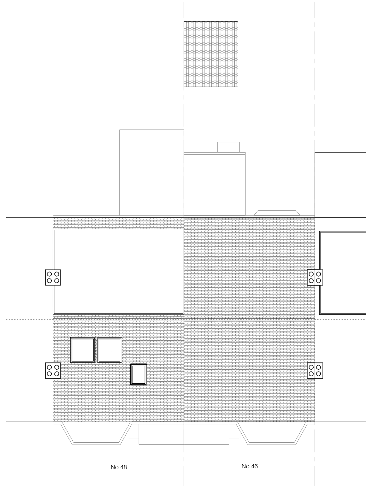
01 Existing Roof Plan
