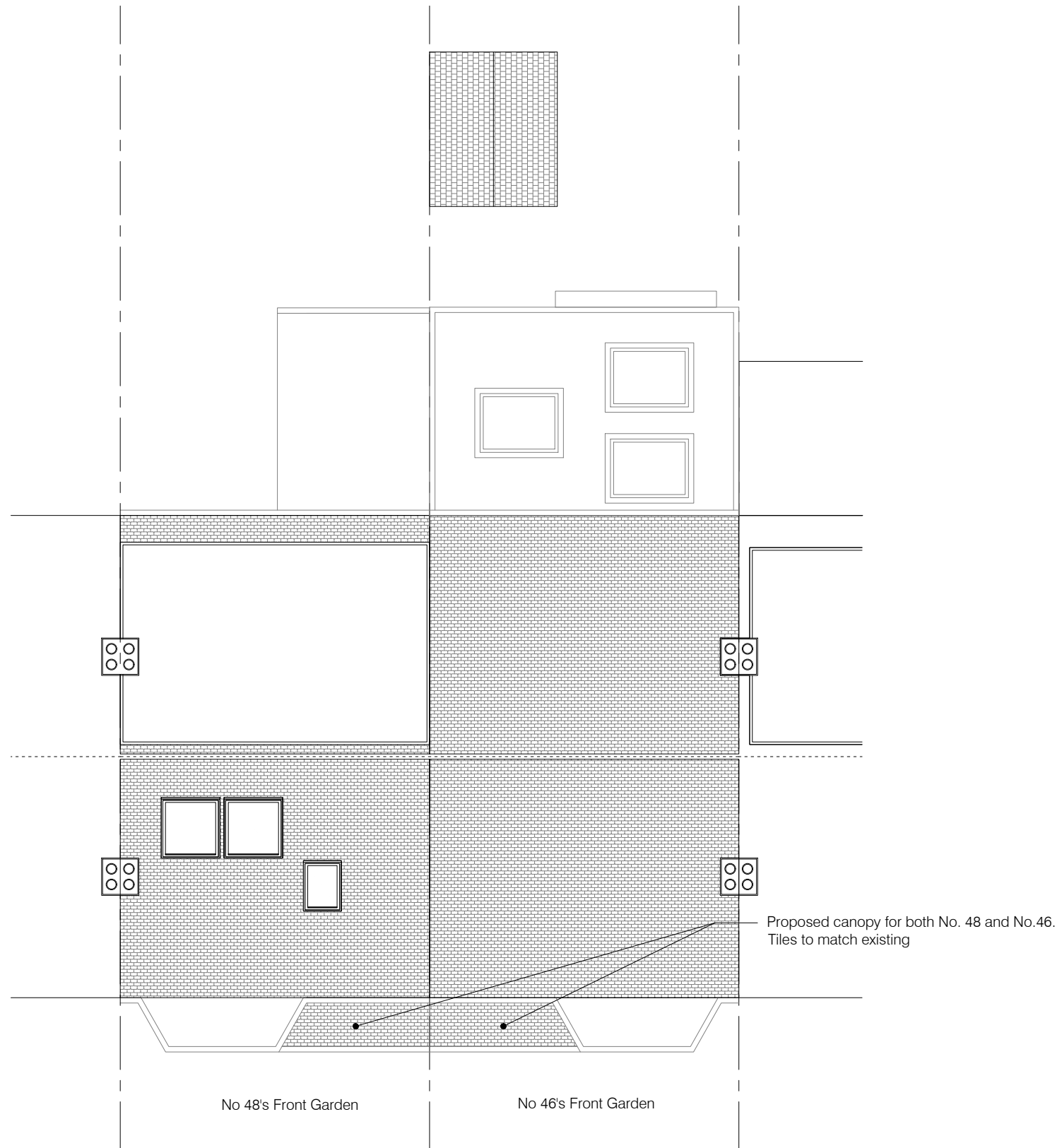
01 Proposed Roof Plan
