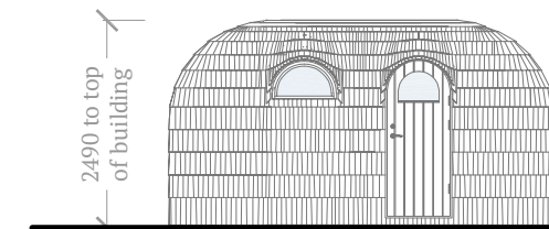
Front (south) Elevation Sauna cabin
