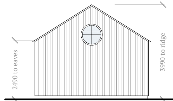
Side (south) Elevation Garden room (home gym/studio)
