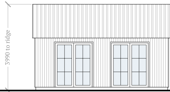
Front (east) Elevation Garden room (home gym/studio)
