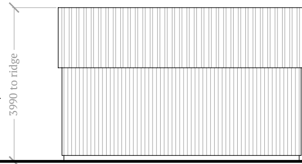
Rear (west) Elevation Garden room (home gym/studio)
