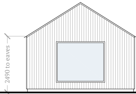
Side (north) Elevation Garden room (home gym/studio)
