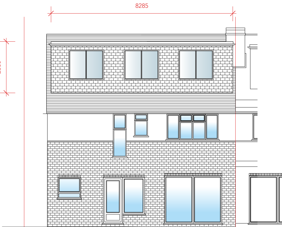
Rear Elevation C
