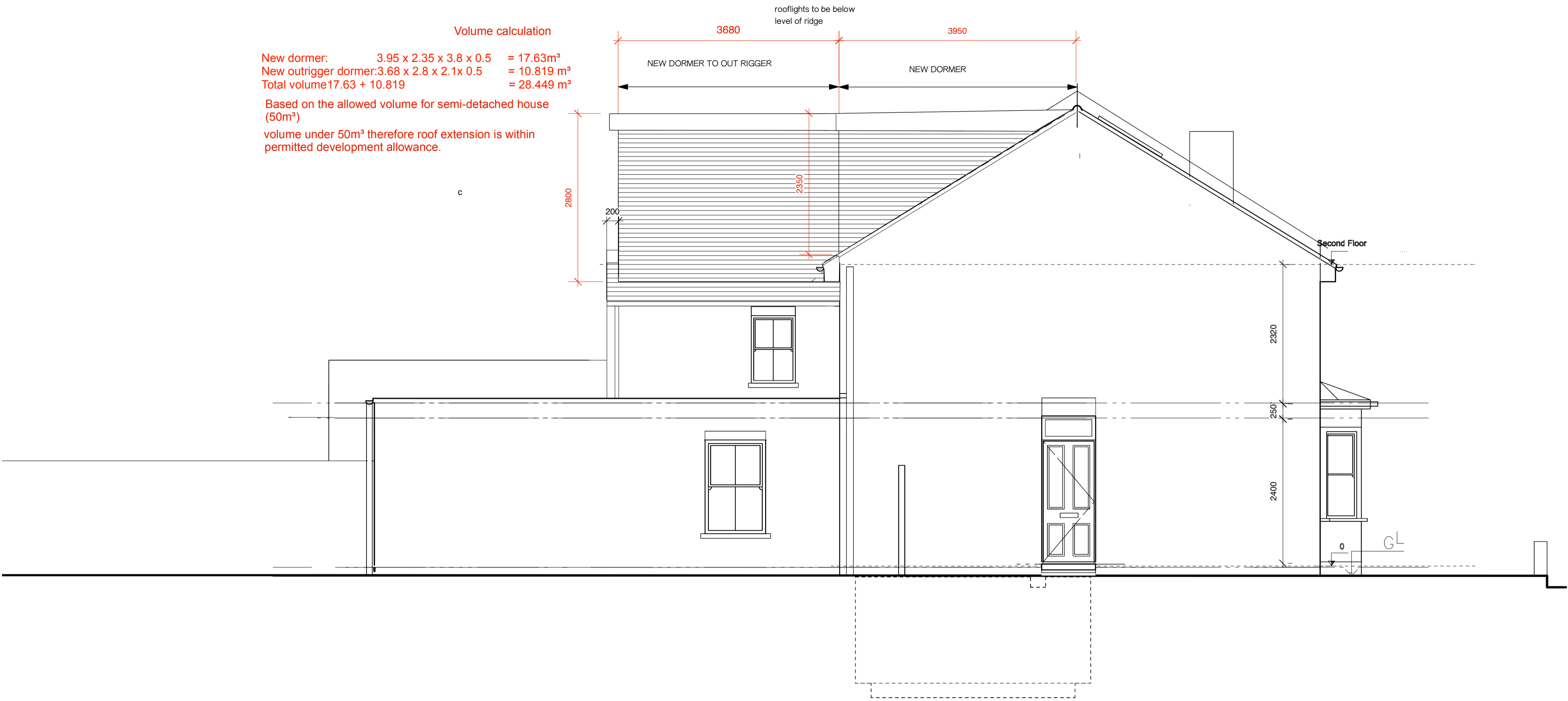
PROPOSED WEST SIDE ELEVATION 1:50
