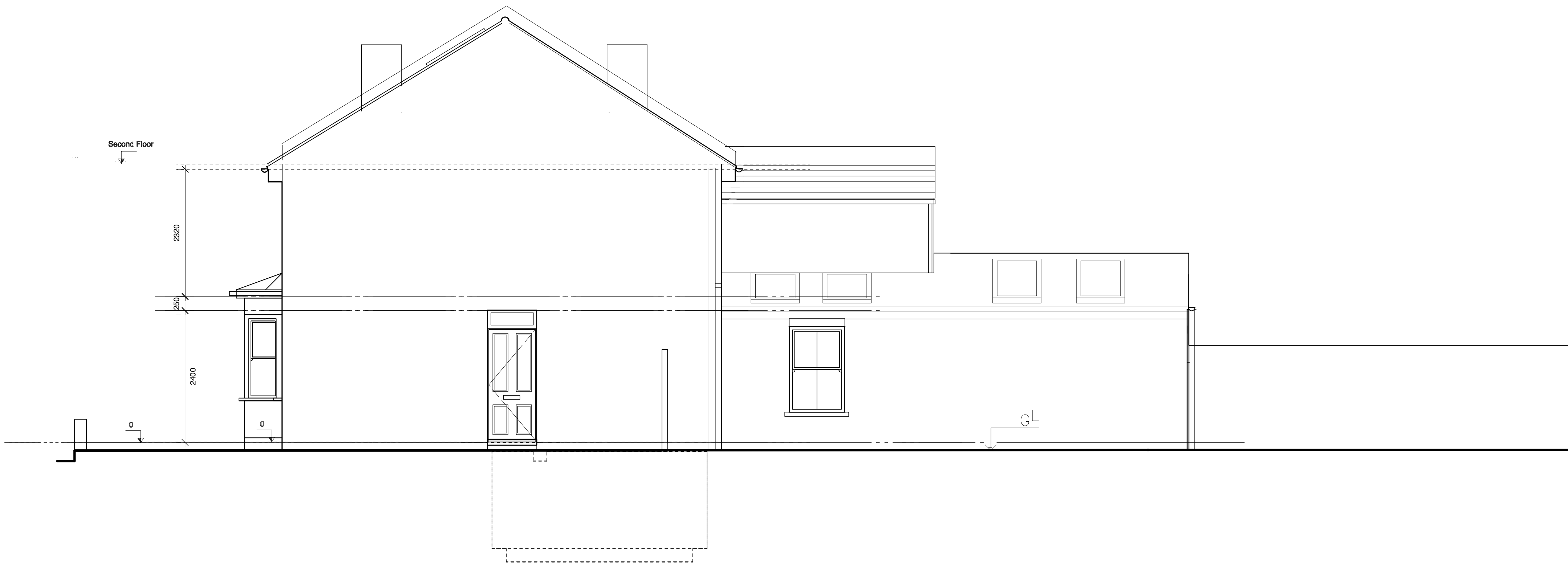
EXISTING EAST SIDE ELEVATION 1:50
