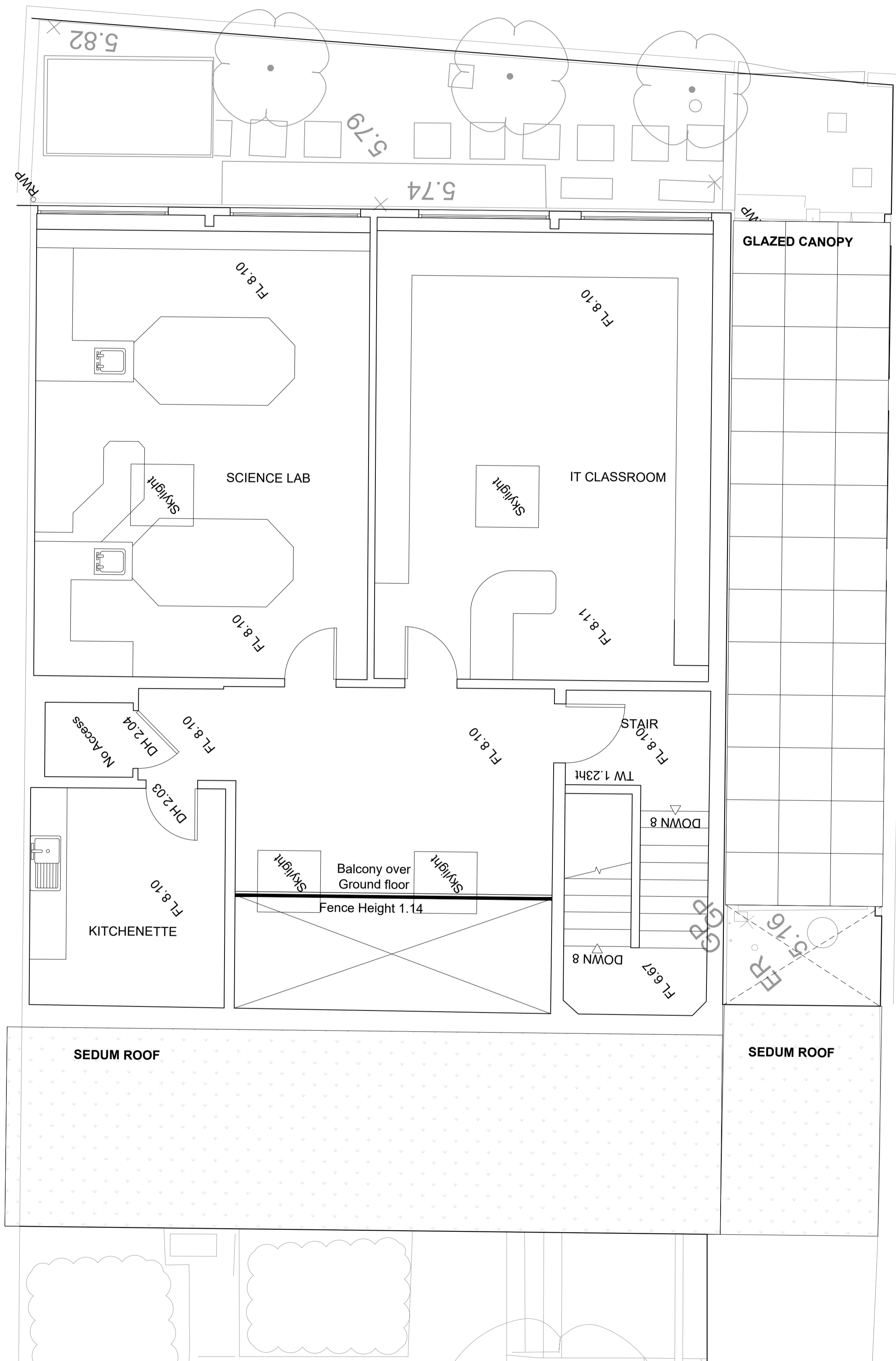
PLN Existing First Floor & Levels Plan 01 Scale 1:50 @ A1
