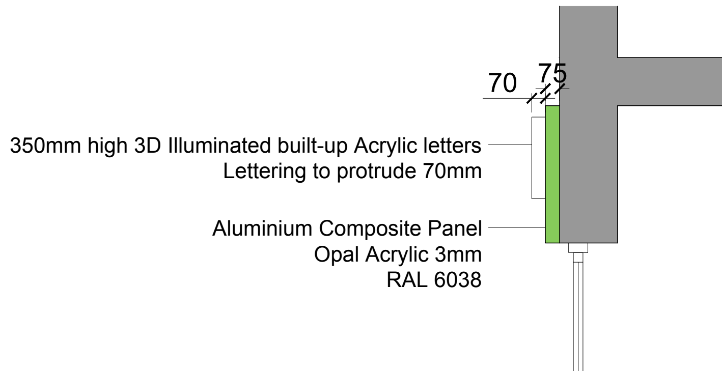
Section through Sign Scale 1:20
