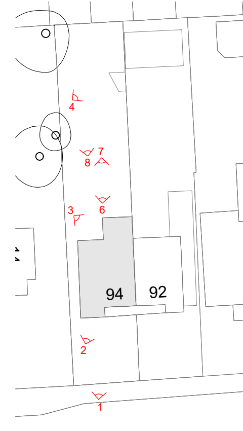
1 Existing Block Plan 1 : 500
