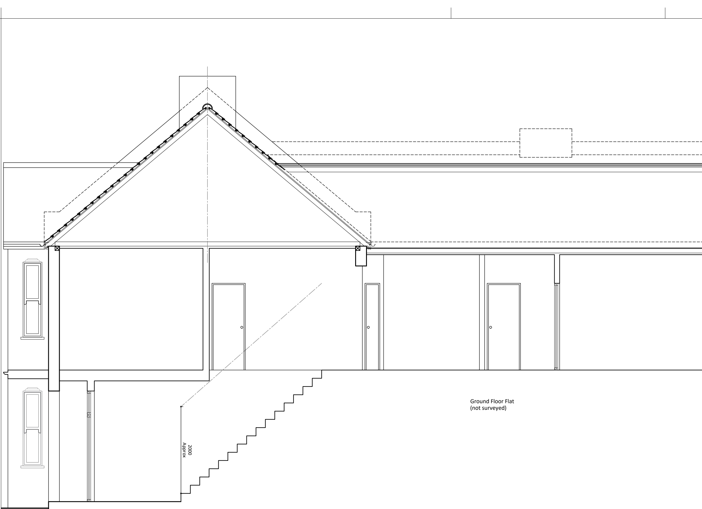
Existing Section A-A Scale 1:50@A3
