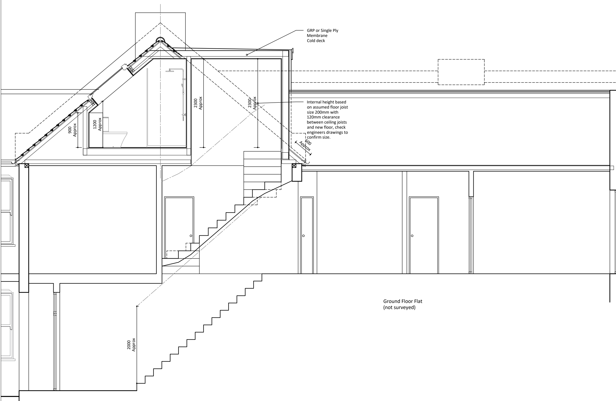
Proposed Section A-A Scale 1:50@A3
