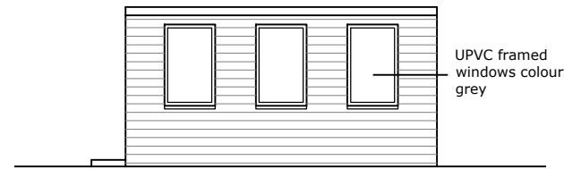
SIDE ELEVATION 1
