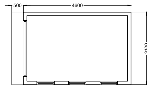
FLOOR PLAN
