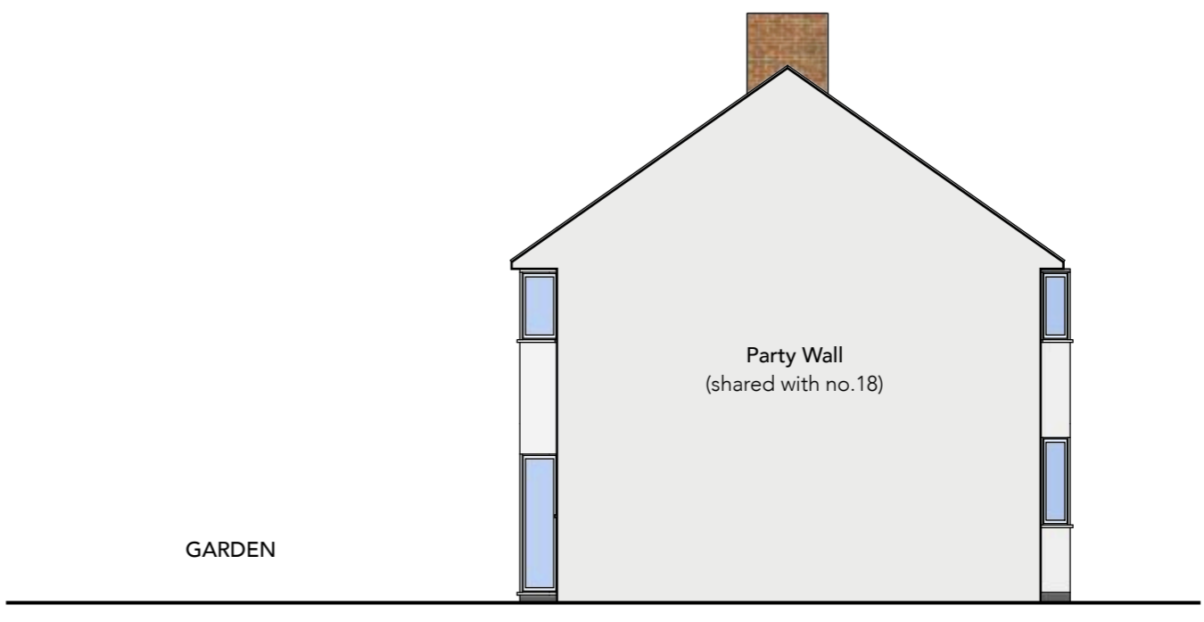
EXISTING SIDE ELEVATION 2
