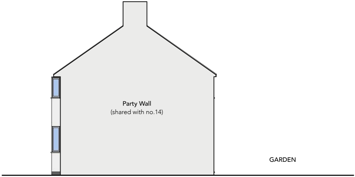
EXISTING SIDE ELEVATION 1
