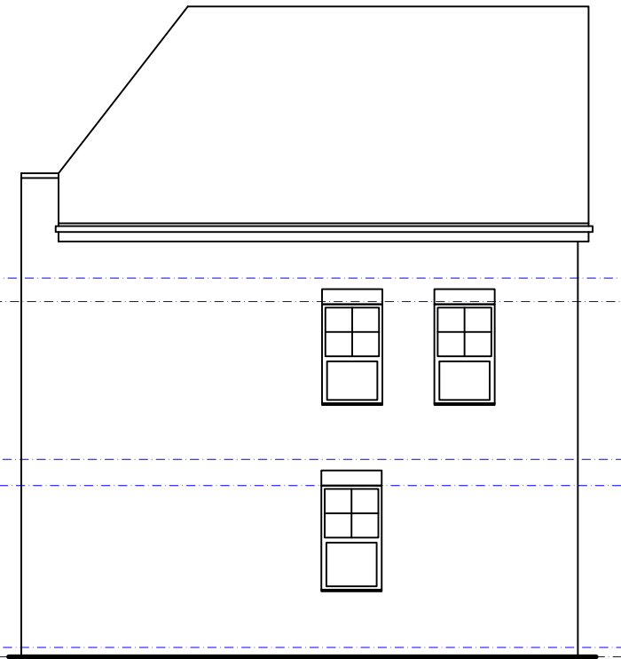
2 EX WEST ELEVATION JARDINE 1:100
