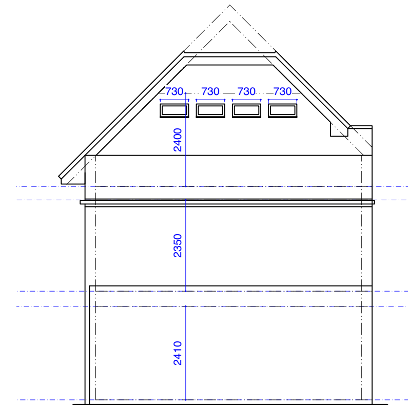
3 PR EAST ELEVATION JARDINE 1:100
