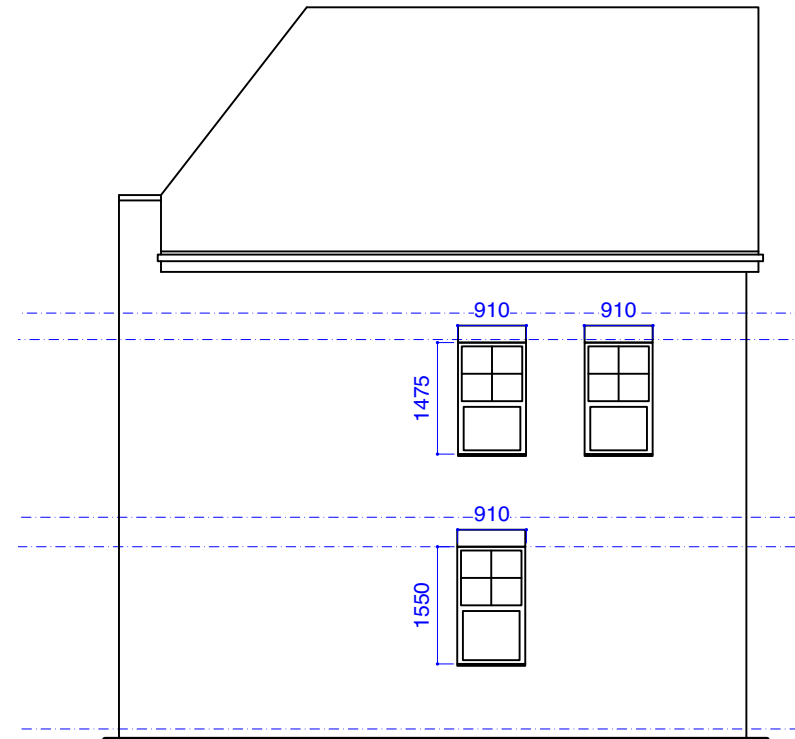
2 PR WEST ELEVATION JARDINE 1:100
