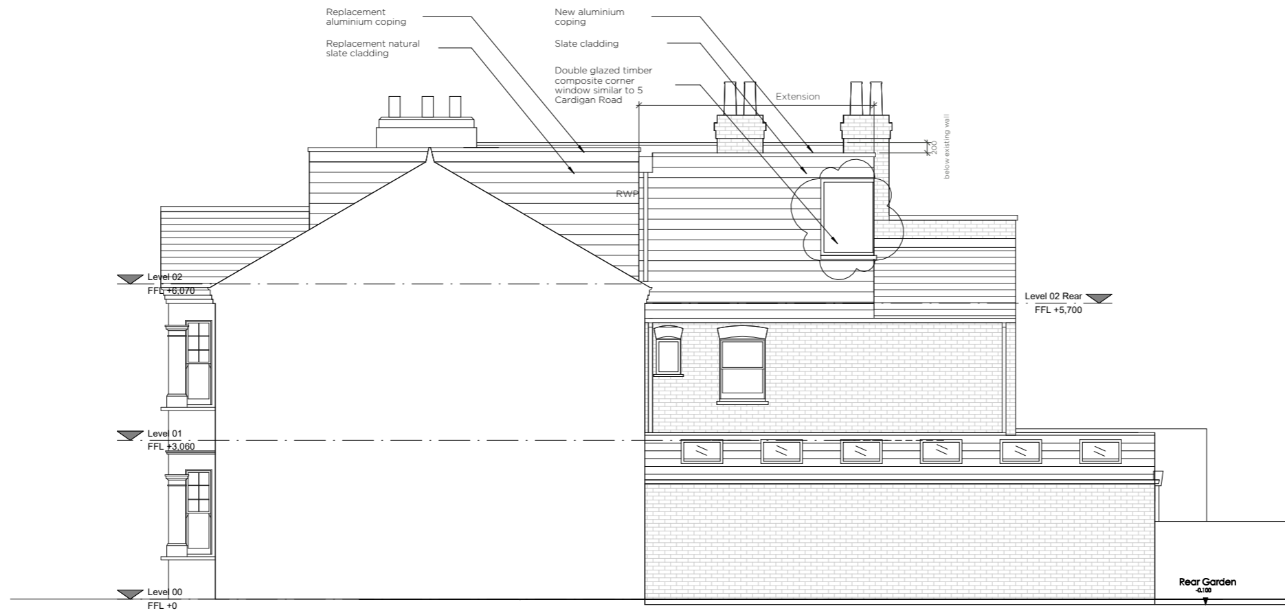
2 | Proposed Elevation-Side Scale 1: 50
