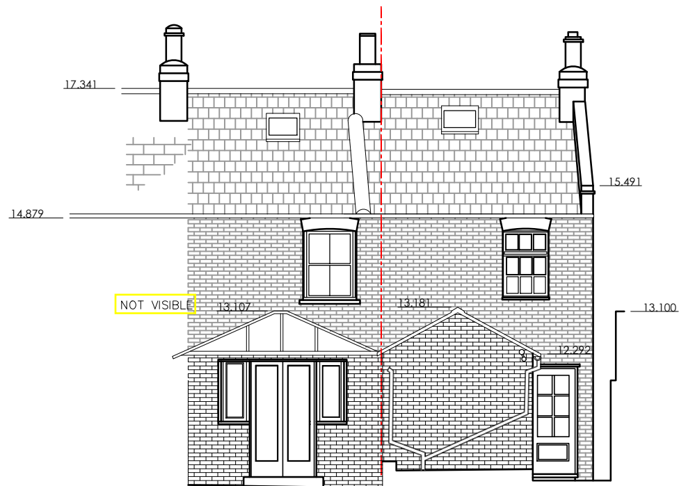
GARDEN ELEVATION
