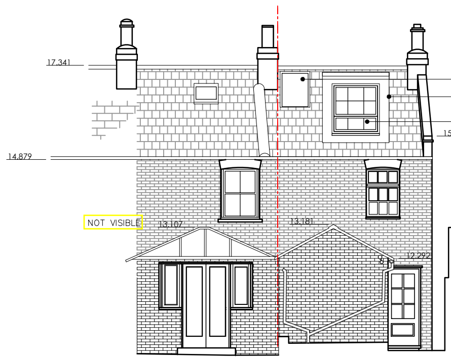
GARDEN ELEVATION
