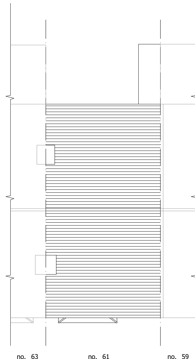
roof plan
