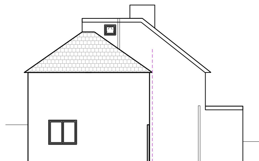
Proposed Elevation
