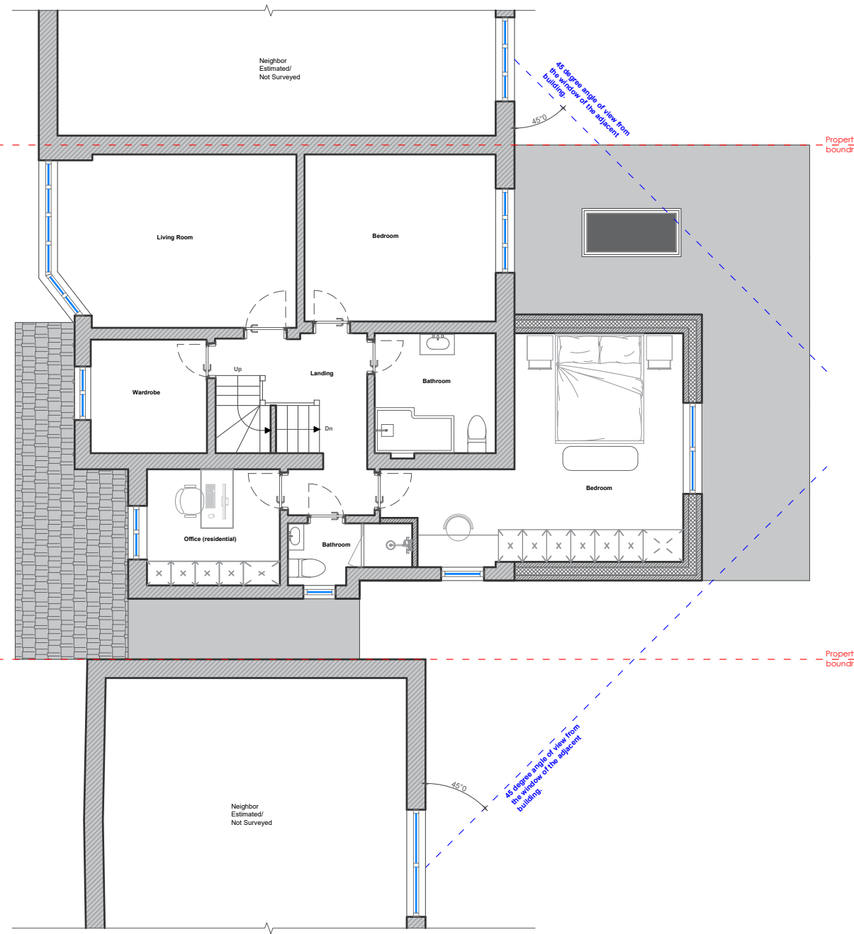
Proposed First 1:100
