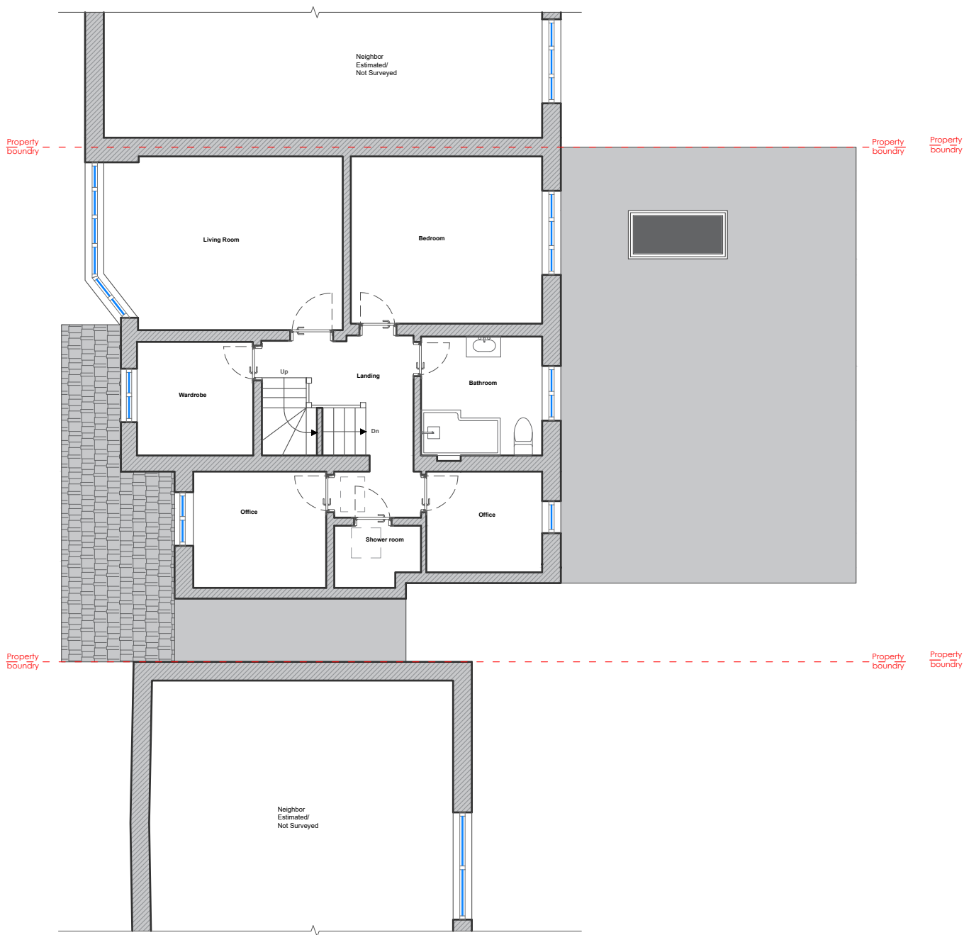
Existing First 1:100
