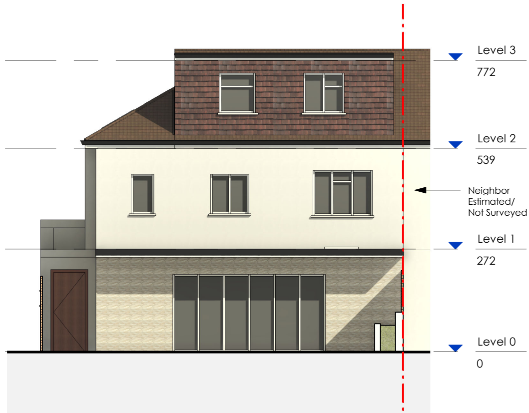
Existing Rear 1:100
