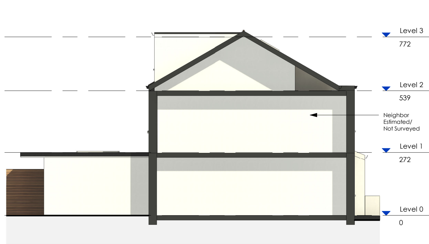
Existing L Side 1:100
