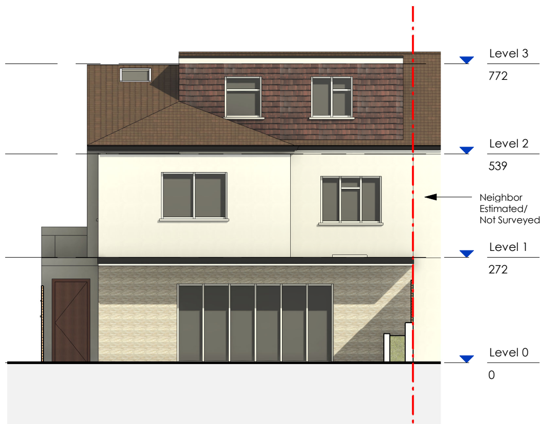
Proposed Rear 1:100
