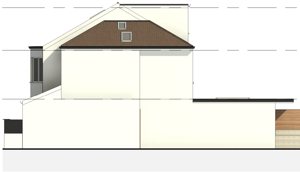
Existing R Side 1:100
