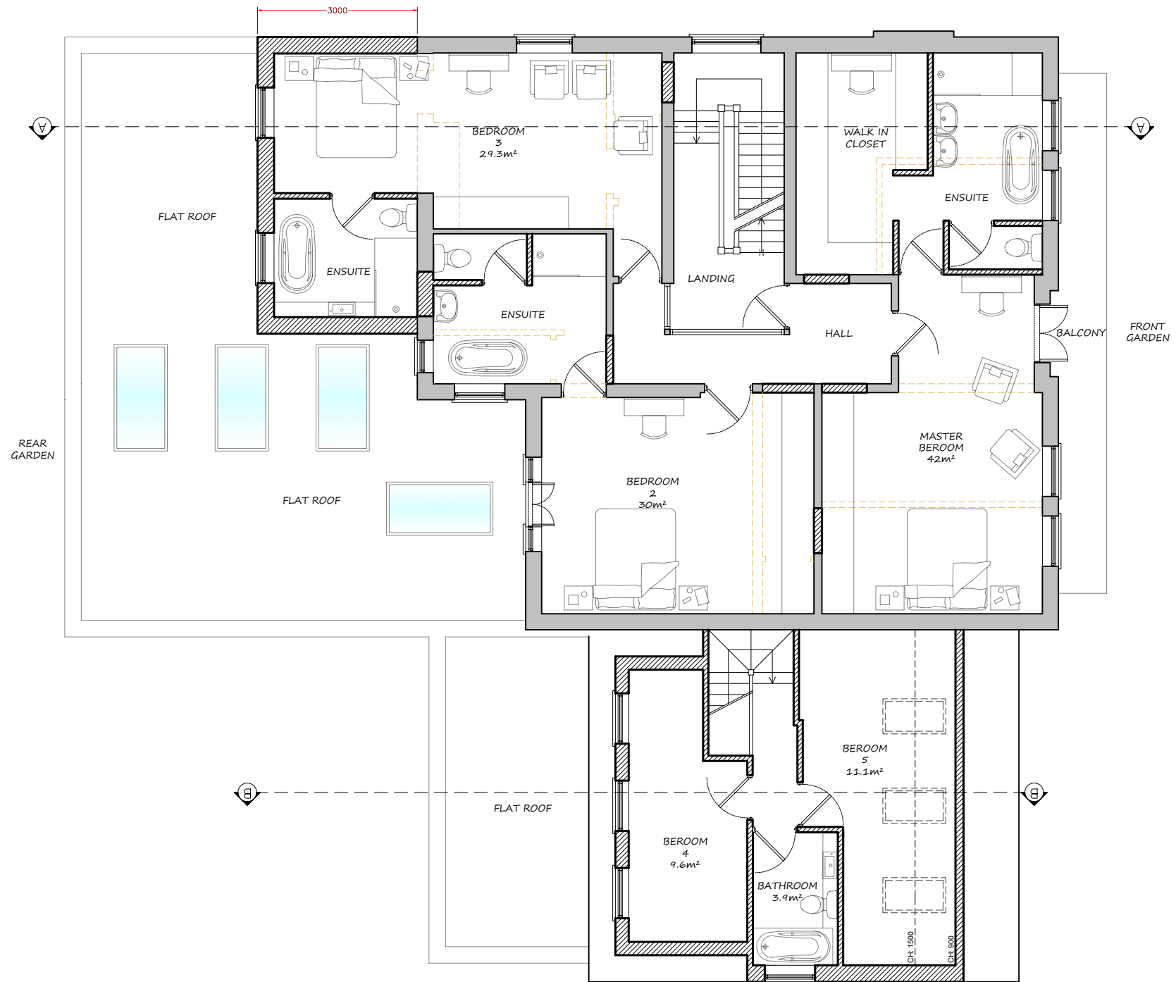
PROPOSED FIRST FLOOR PLAN 1:100
