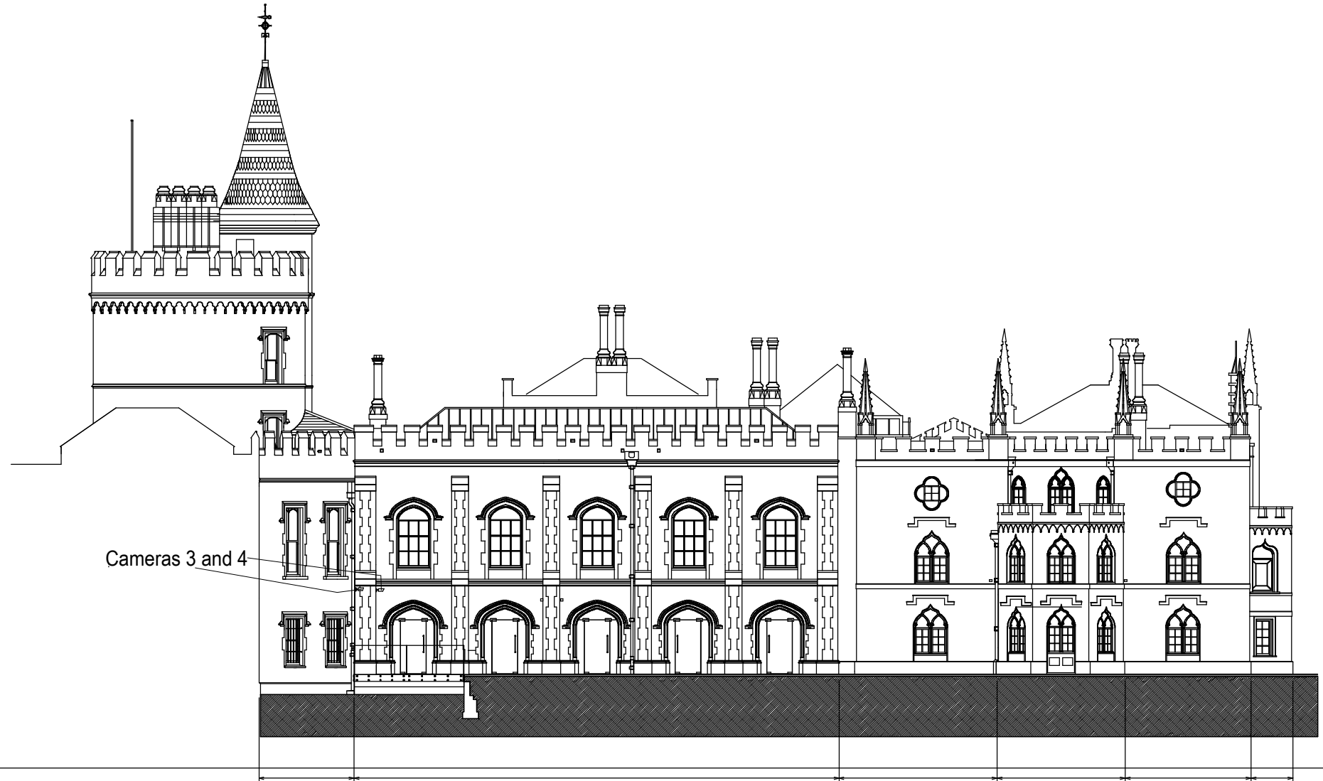
Strawberry Hill House proposed new CCTV cameras South elevation Drg No PC10 scale 1:200 at A4
