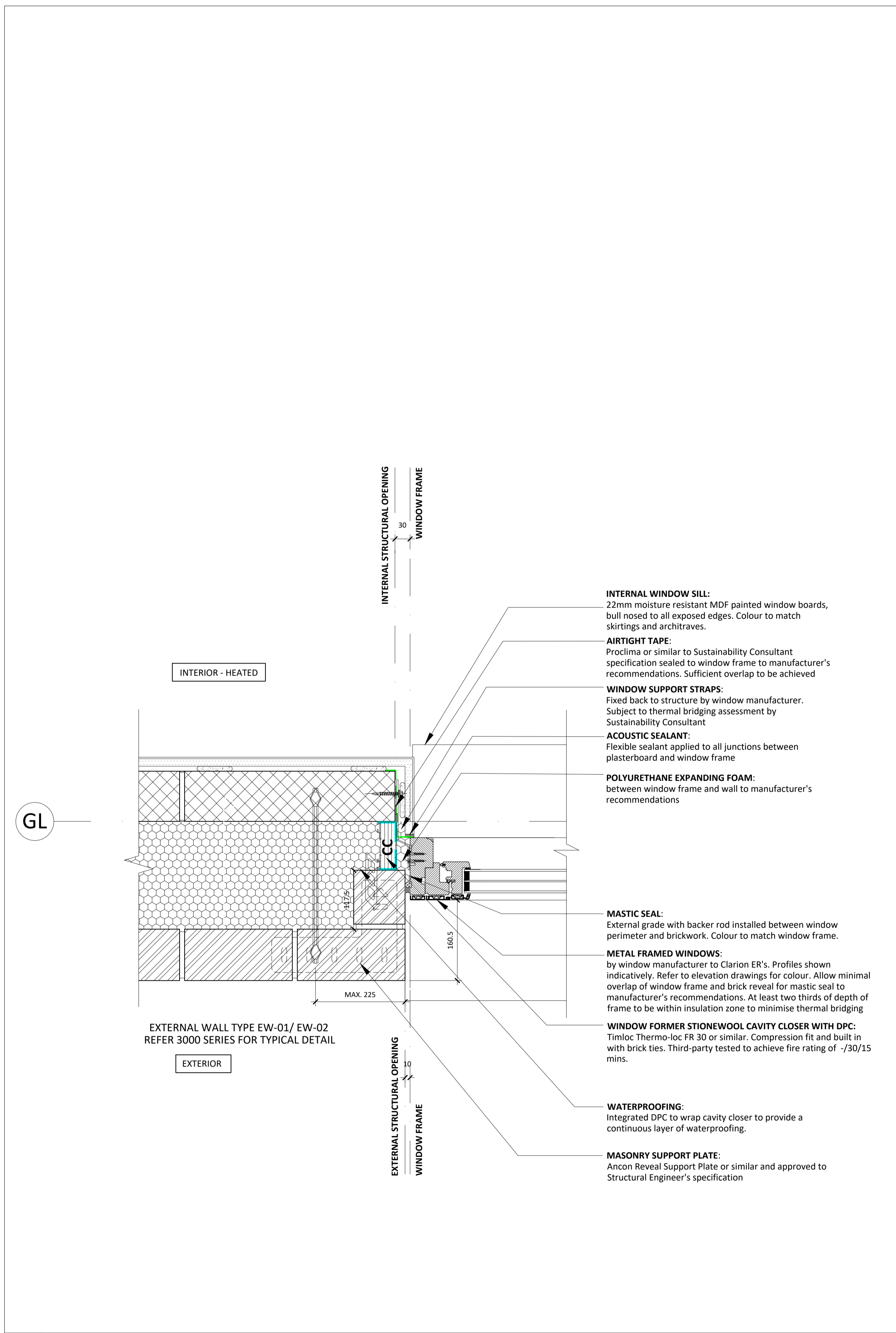
01 Masonry Blocks - Typical Window Jamb 1:5
