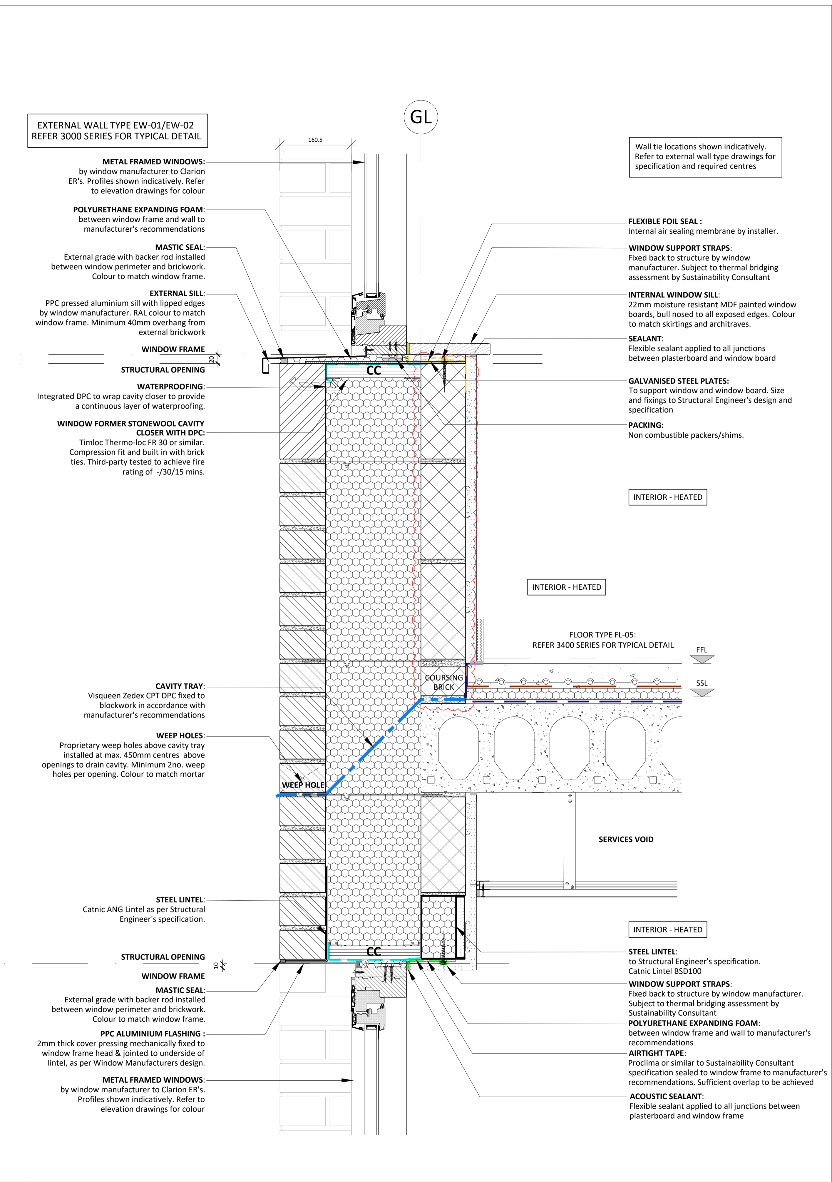
02 Masonry Blocks - Typical Window Head and Sill Detail 1:5
