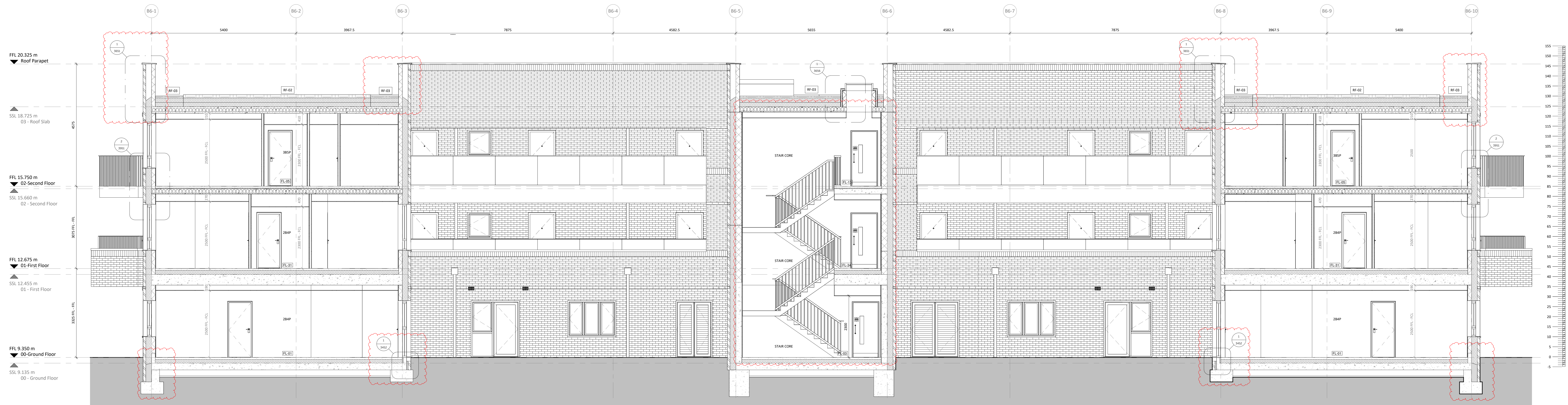
Section B-B 1:50
