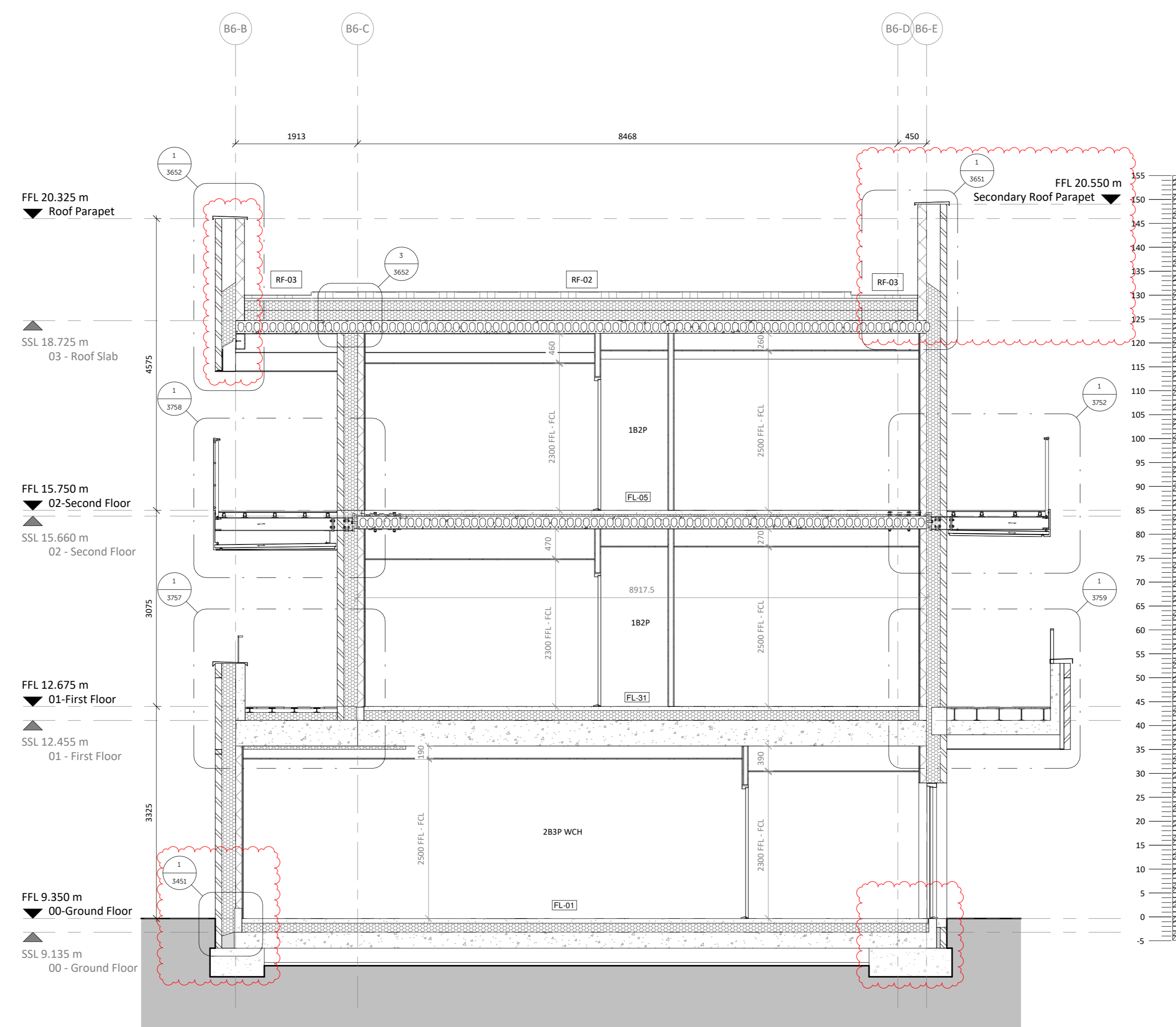
Section C-C 1:50
