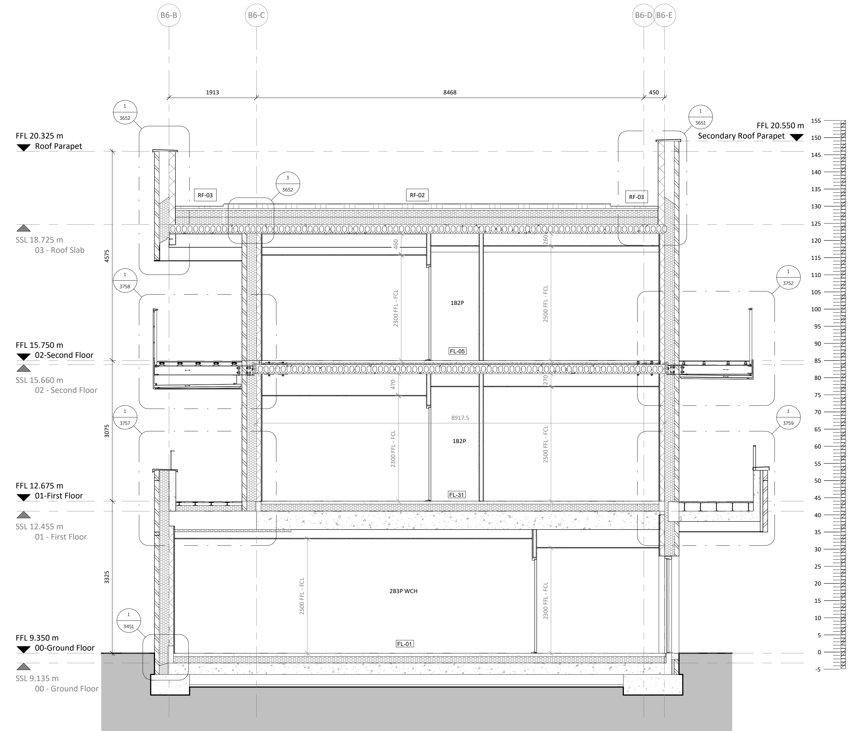
Section C-C 1:50
